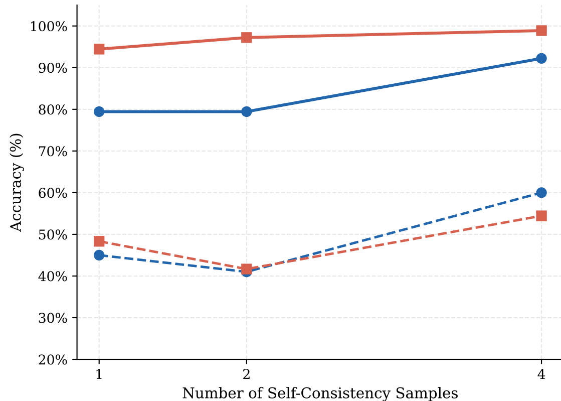
MultiArith
