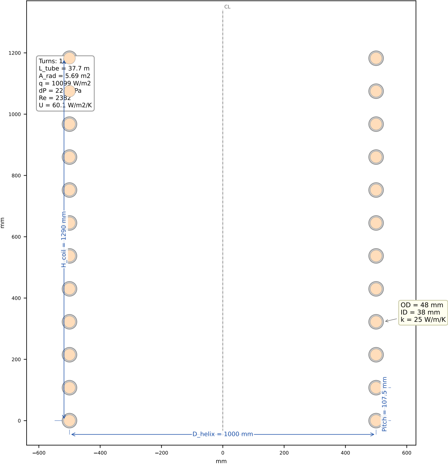
Sheet 6 - Radiant Helical Coil (Side Profile)
