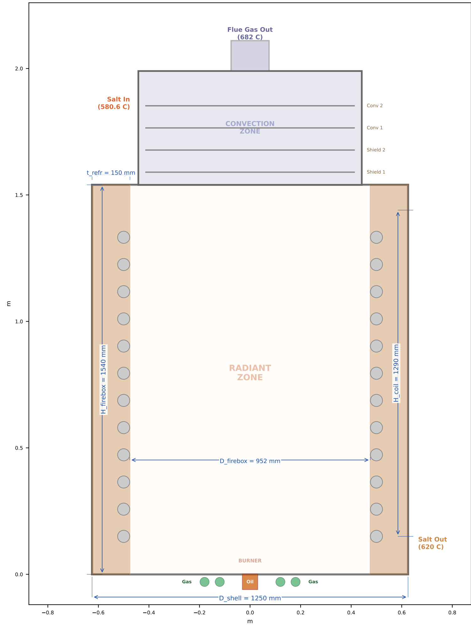
Sheet 1 - Overall Side Elevation (Section A-A)
