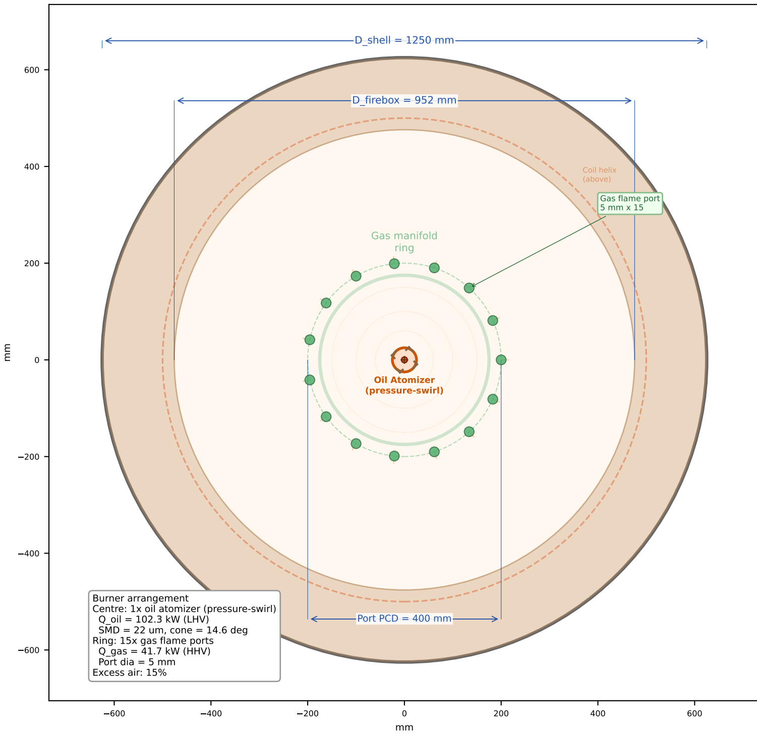
Sheet 2 - Burner Arrangement Plan View (Looking Up)
