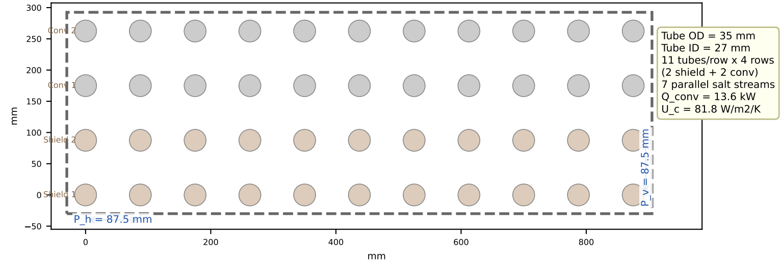
Sheet 5 - Convection Zone Tube Bank (Front View)
