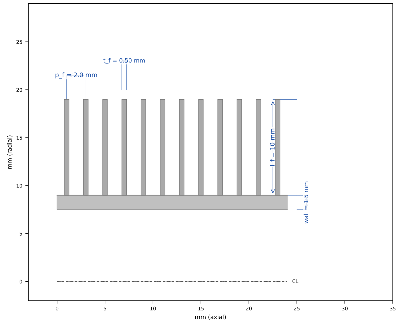
Sheet 3b - Fin Side Profile (Axial Section)
