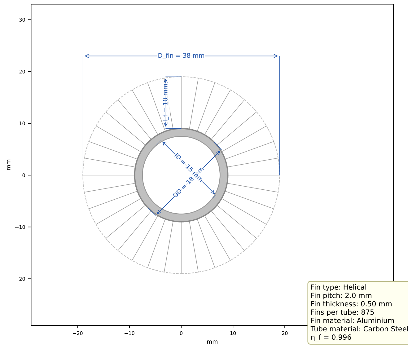
Sheet 3 - Helical Fin Detail
