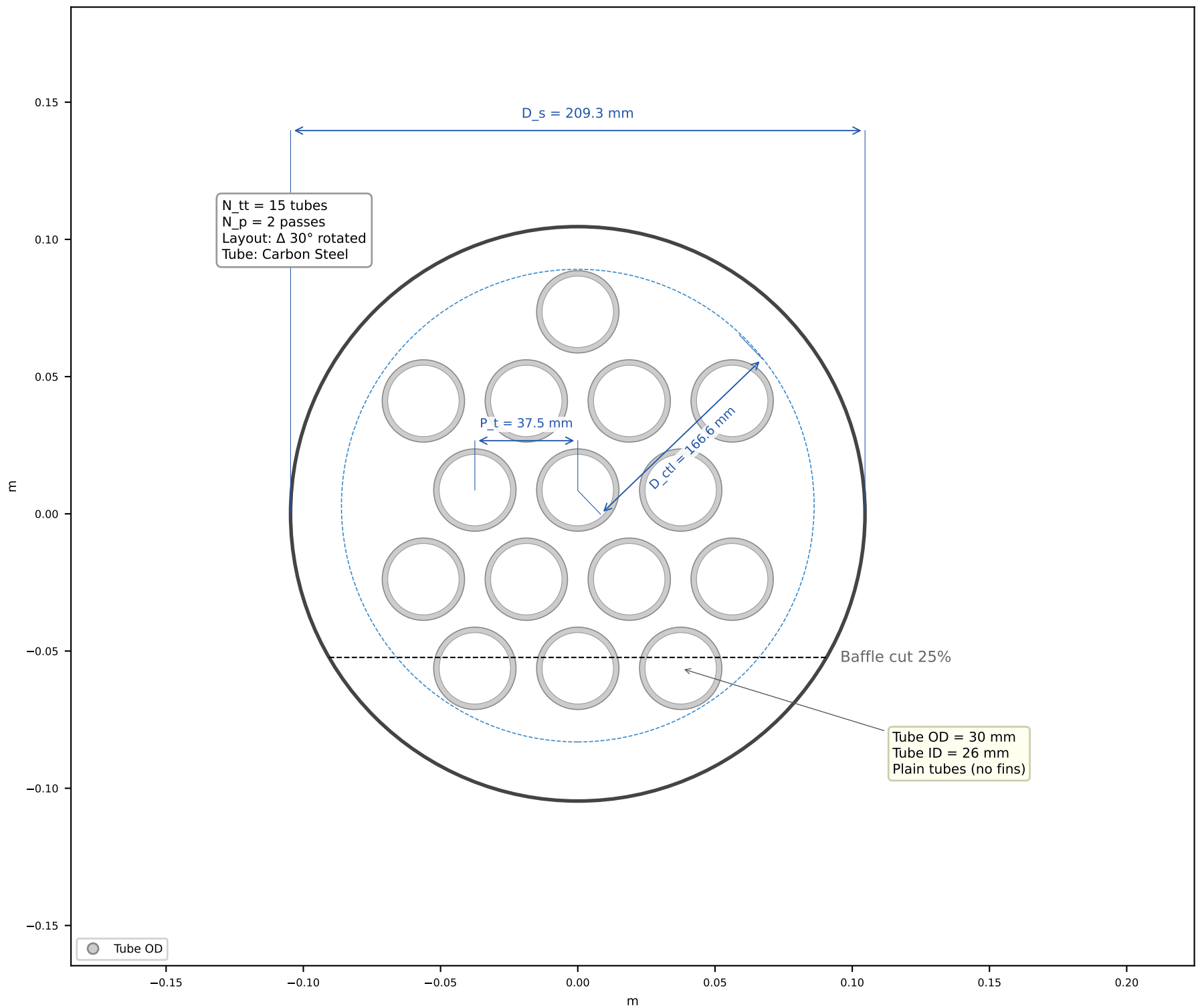
Sheet 1 - Tube-Sheet Cross-Section
