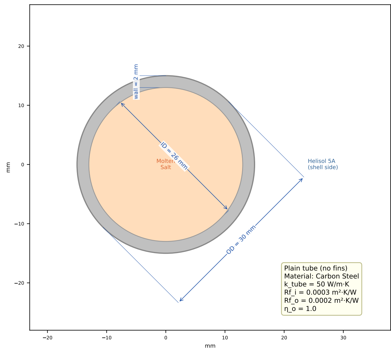
Sheet 3 - Plain Tube Cross-Section Detail
