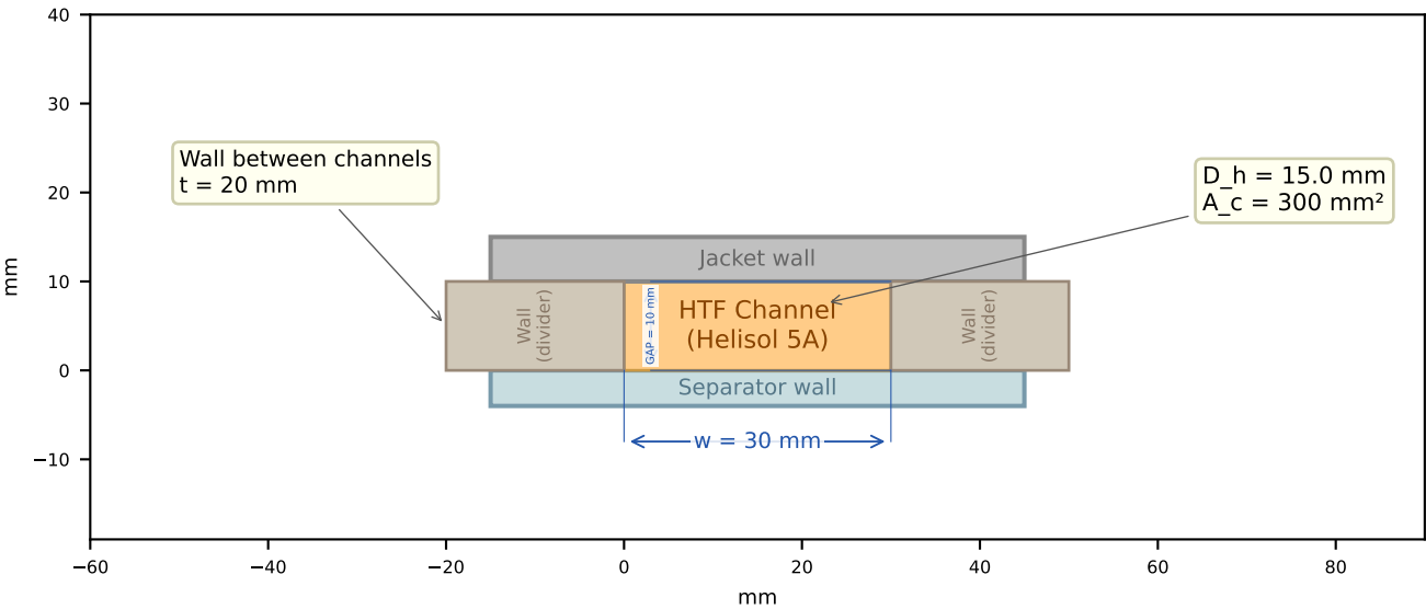
Sheet 3 - Channel Cross-Section Detail
