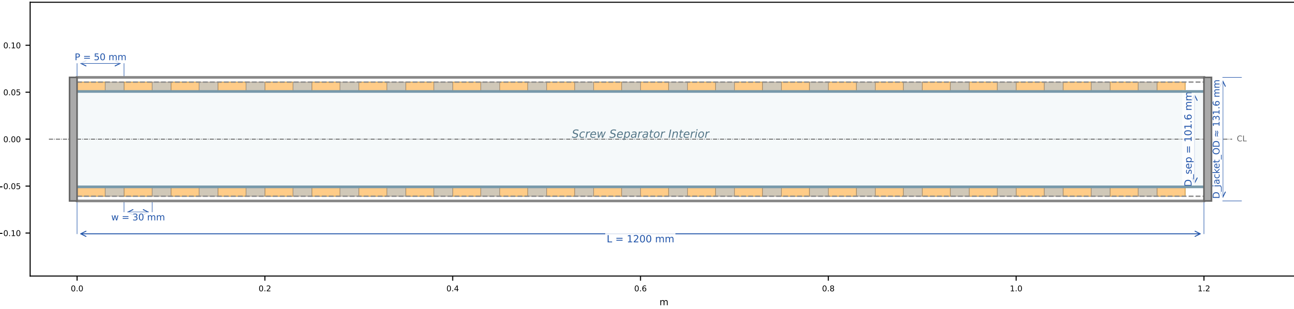
Sheet 2 - Longitudinal Section (Side Elevation)
