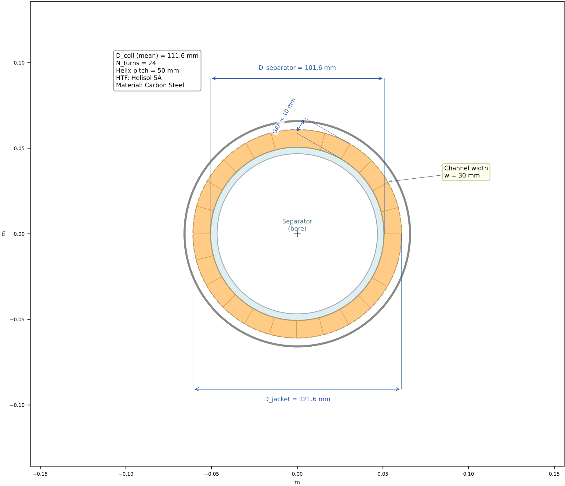
Sheet 1 - Radial Cross-Section (End View)
