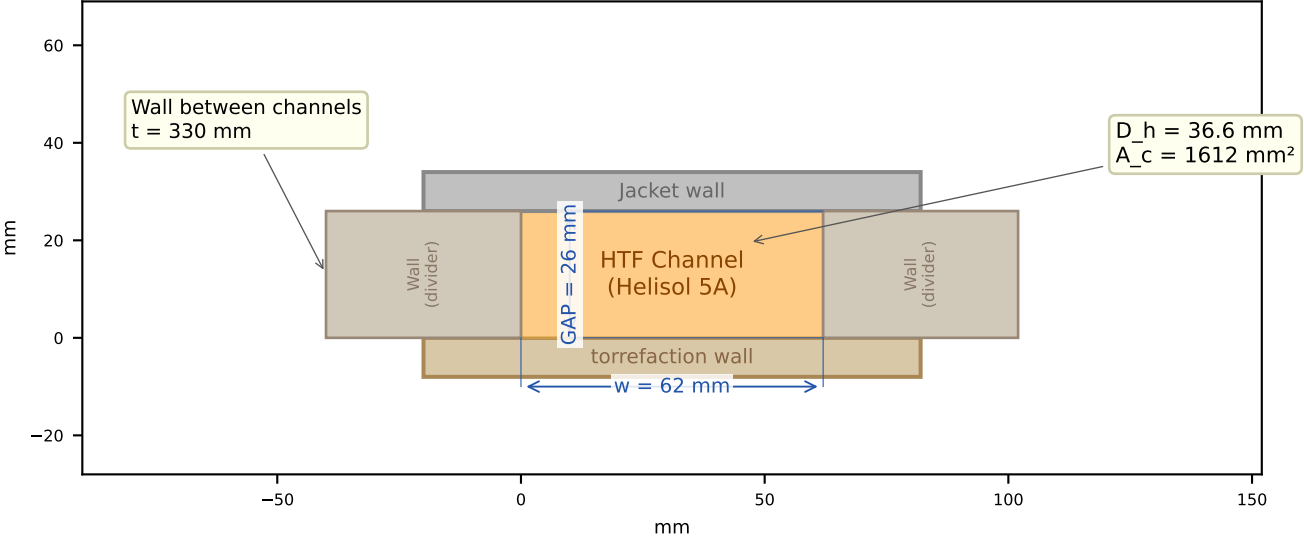
Sheet 3 - Channel Cross-Section Detail
