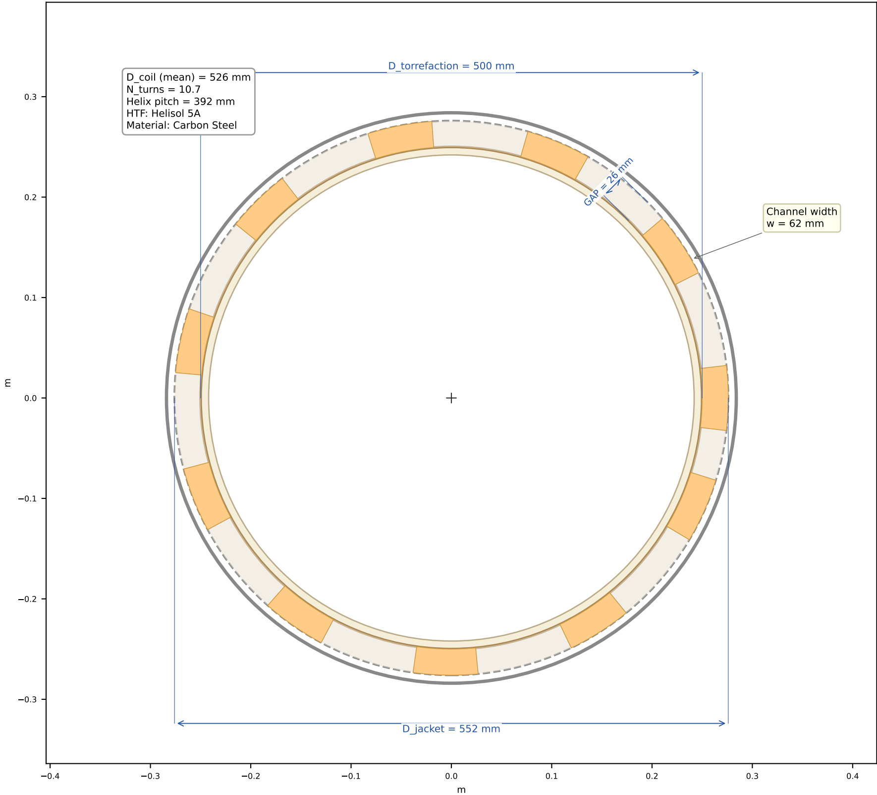
Sheet 1 - Radial Cross-Section (End View)
