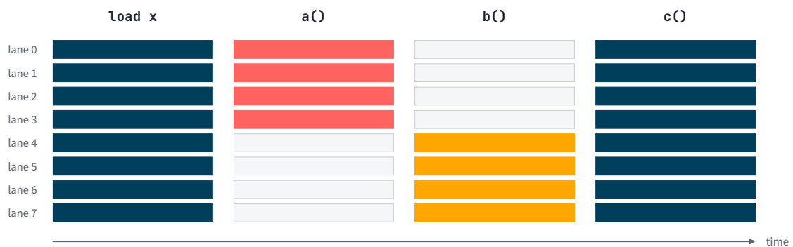
Figure 3.2. Divergence. Eight lanes of a subgroup run an if whose condition differs between lanes: the subgroup runs both branches in turn, with the lanes that did not take each branch masked off.
