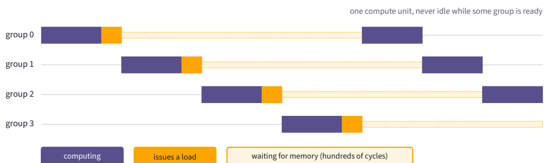
Figure 3.3. Latency hiding. Four subgroups share one compute unit; while each waits for memory, the others compute.
