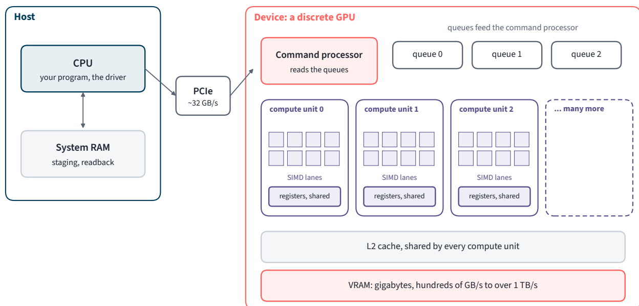
Figure 3.1. Host and device. The host sends work through queues that the GPU's command processor reads; the compute units do the work; every unit shares the L2 cache and the device's memory.
