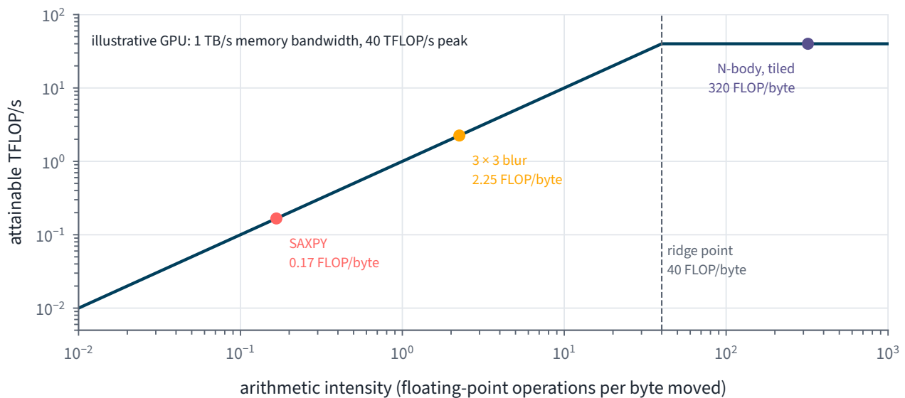
Figure 3.5. The roofline of an illustrative GPU with 1 TB/s of memory bandwidth and 40 TFLOP/s of arithmetic, computed. The kernels are placed by their arithmetic intensity, assuming each byte moves between memory and the GPU once. Chapter 2.5 measures the roofline of your own GPU.
