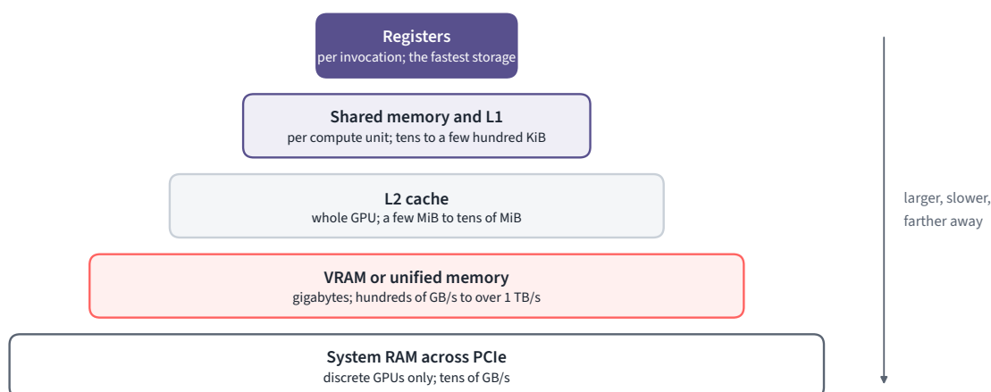
Figure 3.4. The memory hierarchy, from registers to system RAM. Each level is larger, slower and farther from the arithmetic than the one above.
