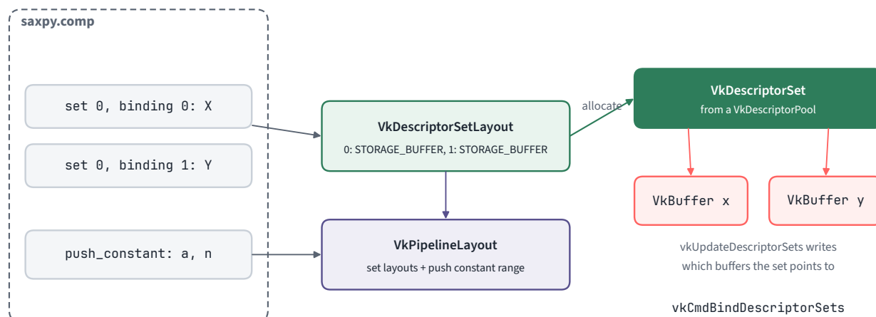
Figure 1.5.1. From the shader's bindings to real buffers. The set layout describes the bindings; the pipeline layout collects set layouts and push constants; a set allocated from a pool is written to point at buffers and bound before the dispatch.
