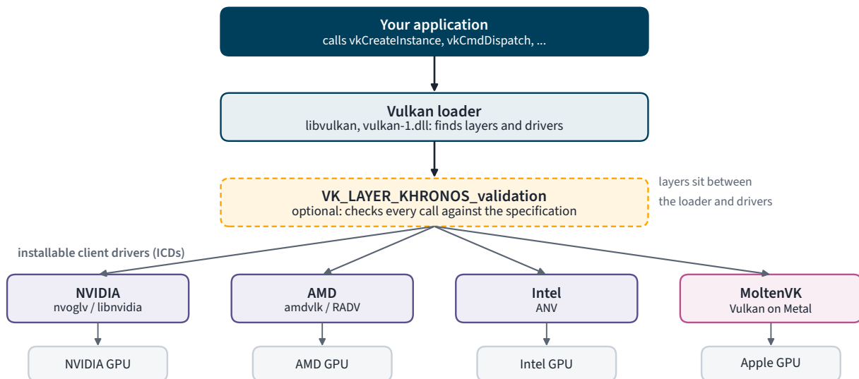
Figure 1.1.2. How a call reaches a GPU. The loader picks the driver for the device you choose and, if you enable it, sends every call through the validation layer first.
