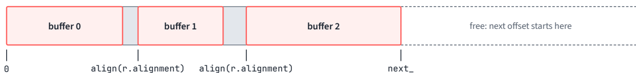
Figure 1.2.2. A linear sub-allocator. Each buffer is placed at the next offset rounded up to its alignment; the grey gaps are the padding that alignment costs.
