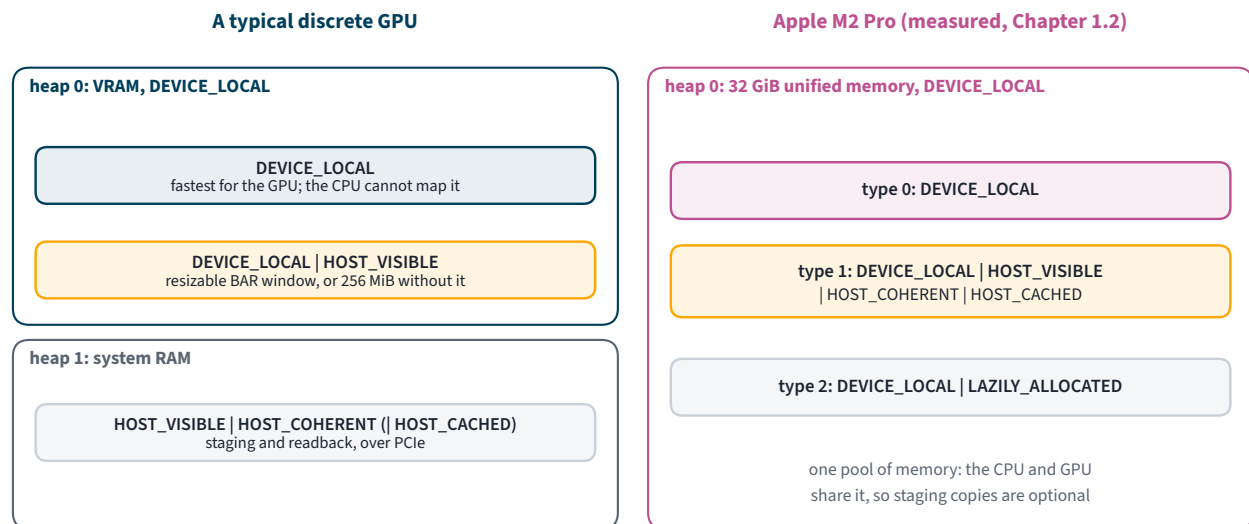
Figure 1.2.1. Heaps and memory types on a typical discrete GPU and on the Apple M2 Pro. Each type is a way of using a heap; the flags tell you who can reach the memory and how fast.
