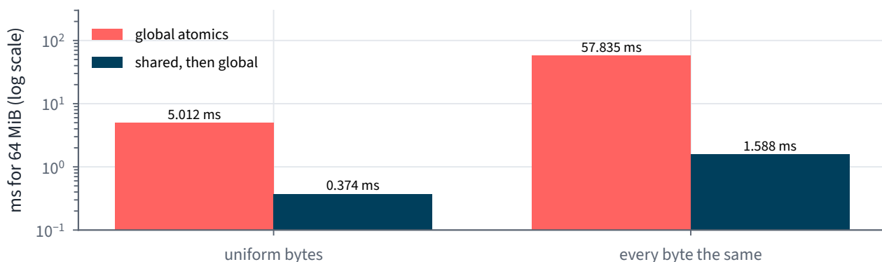
Figure 2.2.4. Time to build the histogram of 64 MiB. Privatisation is about thirteen times faster on random input, and more than thirty times faster when every update hits one bin.
