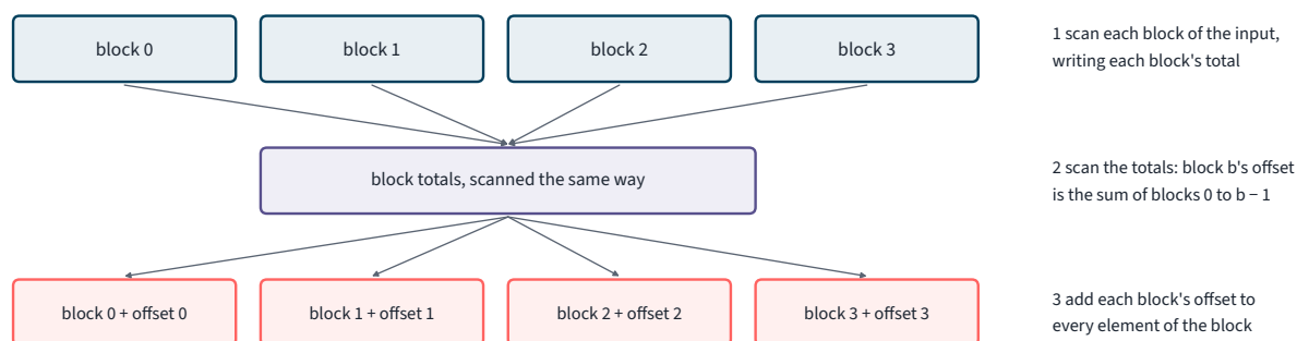
Figure 2.3.4. A multi-level scan. Blocks are scanned independently; the scan of their totals gives each block its offset; adding the offsets completes the scan.
