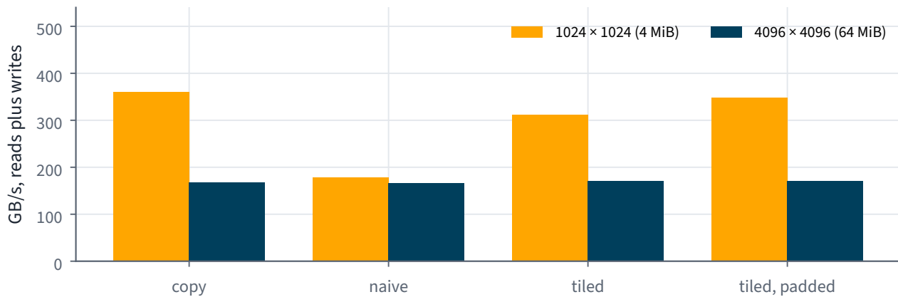
Figure 2.2.2. The transposes on the M2 Pro. With a small matrix, tiling recovers most of what the naive kernel loses; with a large one, every kernel is limited by memory bandwidth.
