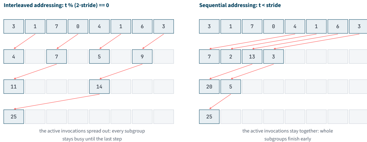
Figure 2.3.1. Two ways to address a tree reduction, shown for eight values. Both perform the same additions; they differ in which invocations do them.
