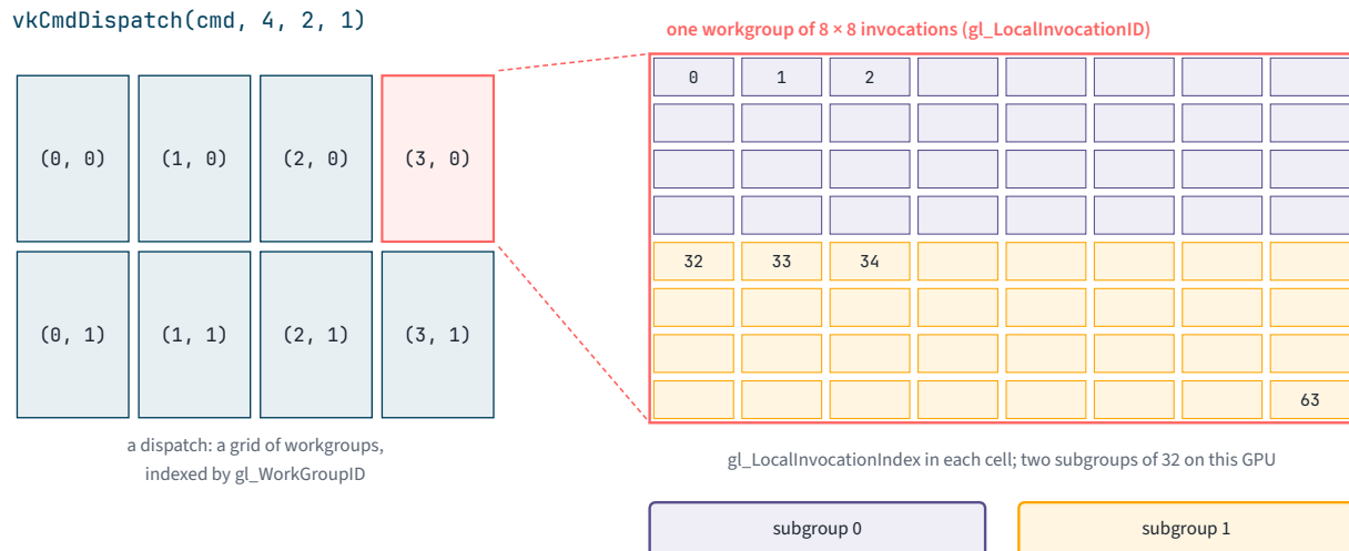
Figure 2.1.1. A dispatch of 4 \times 2 workgroups, each of 8 \times 8 invocations. On the M2 Pro each workgroup is divided into two subgroups of 32 invocations.
