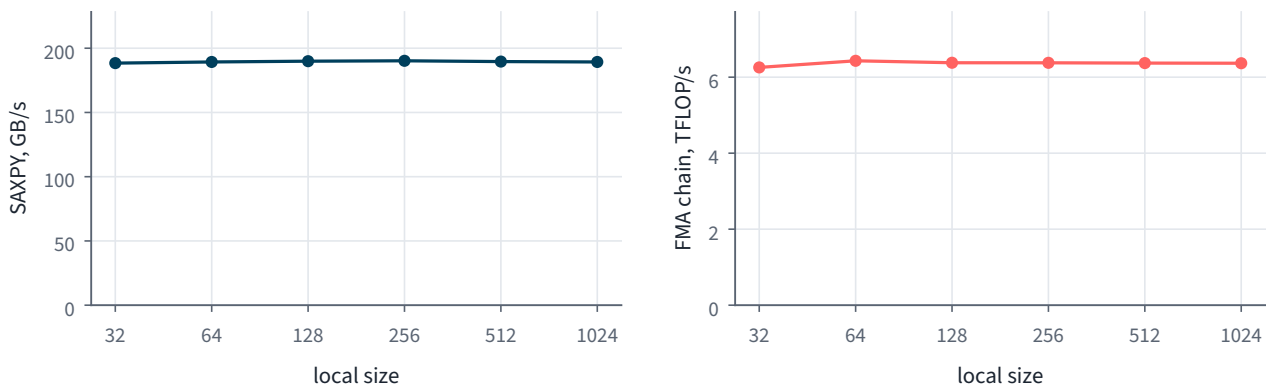
Figure 2.1.2. The sweep plotted. SAXPY is limited by memory bandwidth and reaches about 180 GB/s from 64 invocations up; the chain of multiply-adds is limited by arithmetic and barely notices the local size.
