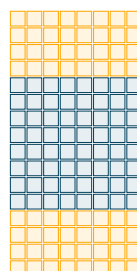
Figure 2.4.1. The data each pass loads into shared memory: the tile it writes, plus aprons wide enough for the blur's radius in the direction of the pass.
