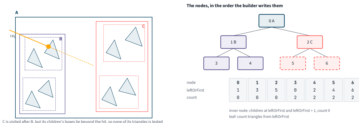
Figure 2.7.1. A hierarchy over eight triangles. Traversal visits the nearer of two children first, and the closest hit found there lets it skip the boxes of the farther one.
