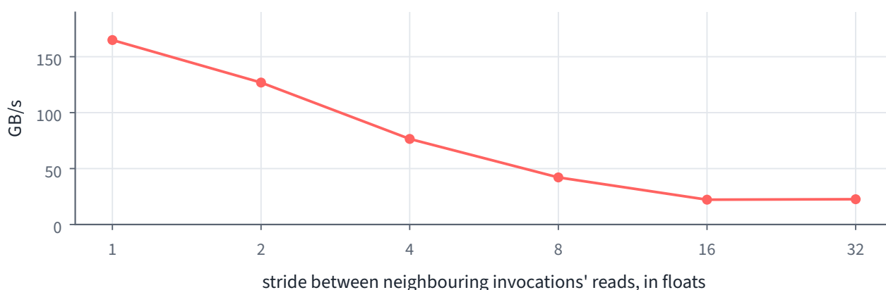
Figure 2.5.1. Bandwidth against the stride between neighbouring invocations' reads, on the M2 Pro.
