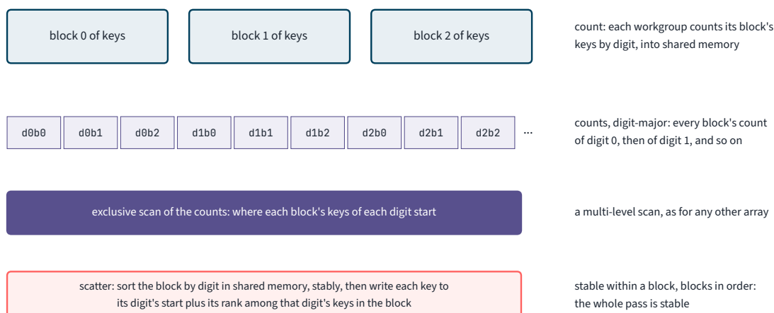
Figure 2.3.5. One pass of the radix sort. Counting and scanning give each block a starting position for each digit; the scatter writes each block's keys there in a stable order.
