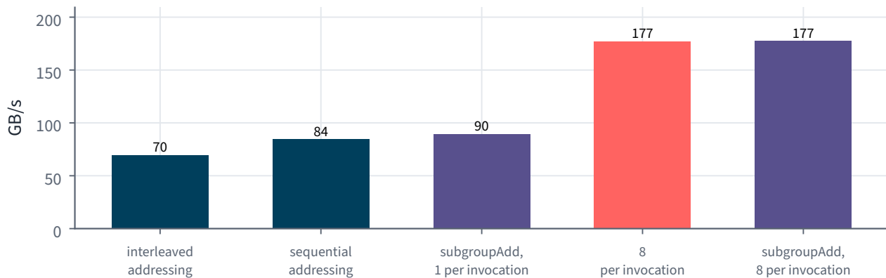
Figure 2.3.2. The reductions' bandwidth on the M2 Pro. Coarsening doubles the speed of either kind of tree; the choice of tree matters little once it does.
