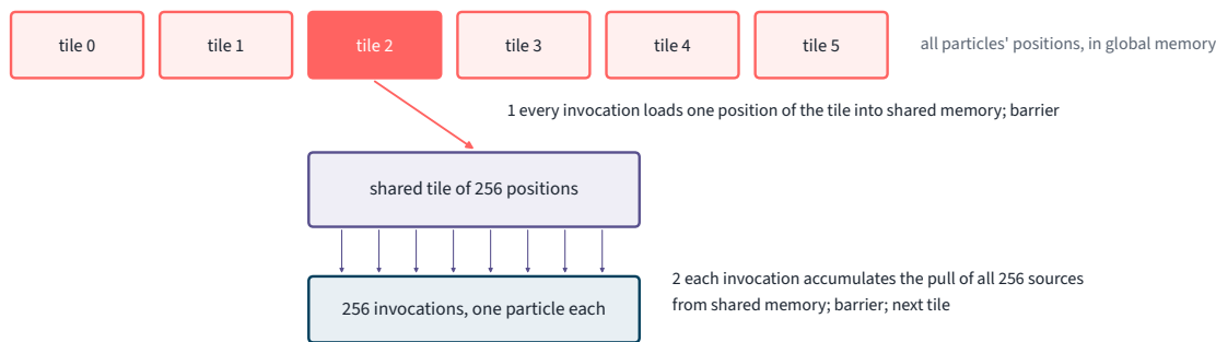
Figure 2.6.1. The tiled force calculation. Shared memory turns 256 reads of each position into one.
