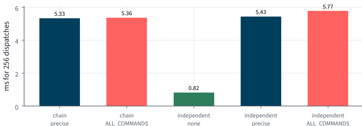
Figure 3.3.2. 256 dispatches of 16,384 elements on the M2 Pro. Any barrier makes each dispatch cost about 20 \mu s; without barriers, independent dispatches overlap and cost about 3 \mu s each.
