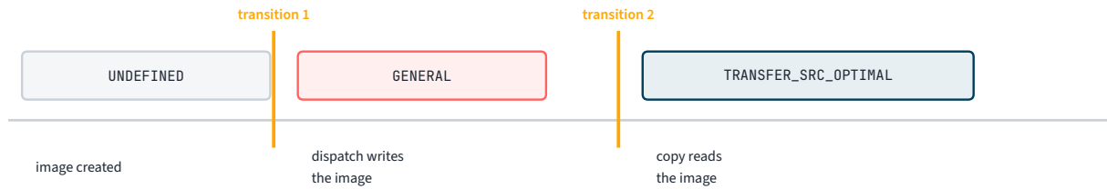
Figure 3.2.3. The image in Chapter 3.1's image-layout case. Each transition belongs to a barrier and sits between that barrier's two scopes.
