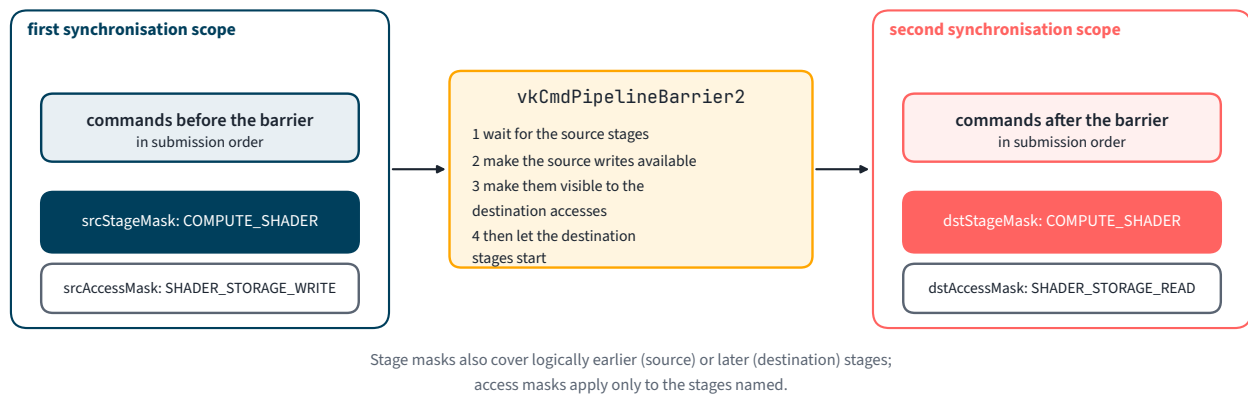
Figure 3.2.1. What a pipeline barrier does. Work in the first scope finishes and its writes in the first access scope are made available and then visible to the second access scope, before work in the second scope starts.
