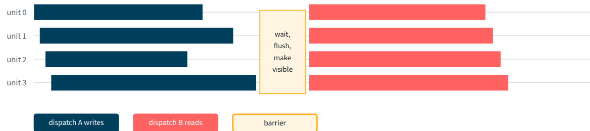
Figure 3.1.1. Two dispatches on four compute units. Without a barrier, B's workgroups start on each unit as soon as A's leave it, while A is still running elsewhere. With a barrier, B waits until A has finished everywhere and A's writes have been made visible.
