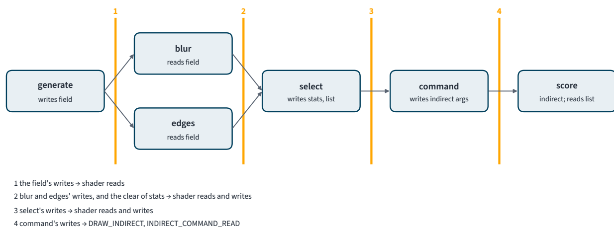
Figure 3.3.1. The pipeline and its four barriers between passes. Before them, a transition takes the field's image from UNDEFINED to GENERAL ; after them, two barriers carry the statistics to a copy and then to the host.
