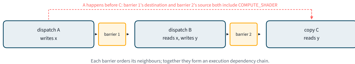
Figure 3.2.4. An execution dependency chain. A happens before B by barrier 1 and B before C by barrier 2; because both barriers include the compute stage between them, A also happens before C.
