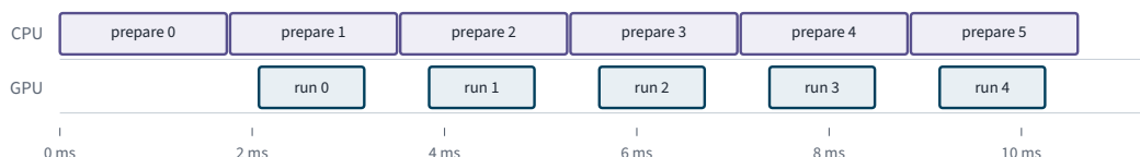
Figure 3.6.1. The measured frame times as a timeline. With one frame in flight a frame costs the CPU's time plus the GPU's, and more; with two it costs the larger of the two.
