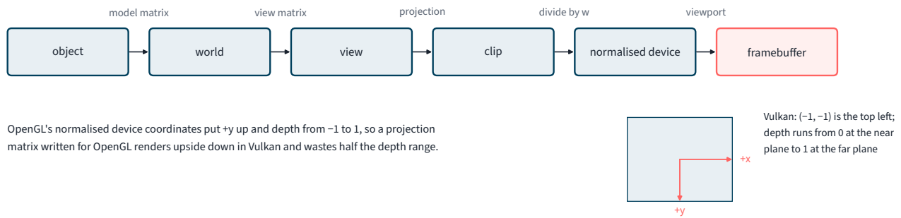
Figure 4.1.2. From an object's coordinates to the framebuffer. Vulkan's normalised device coordinates differ from OpenGL's in two ways that every projection matrix must respect.
