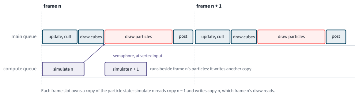
Figure 4.7.1. The passes of two frames on the two queues. The next frame's simulation can run while this frame draws its particles, because it writes another copy of the state.
