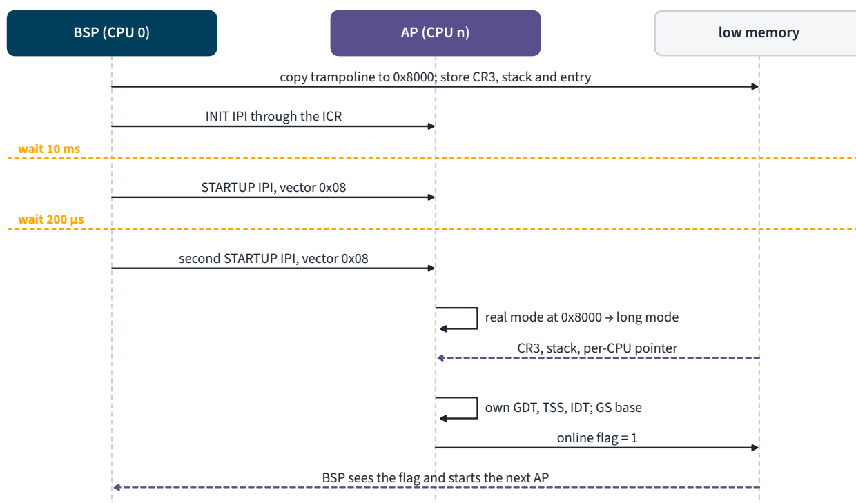
Figure 4.1.3. Bringing up one application processor. The trampoline's data area carries the page-table root and stack that the AP needs to reach long mode and C.
