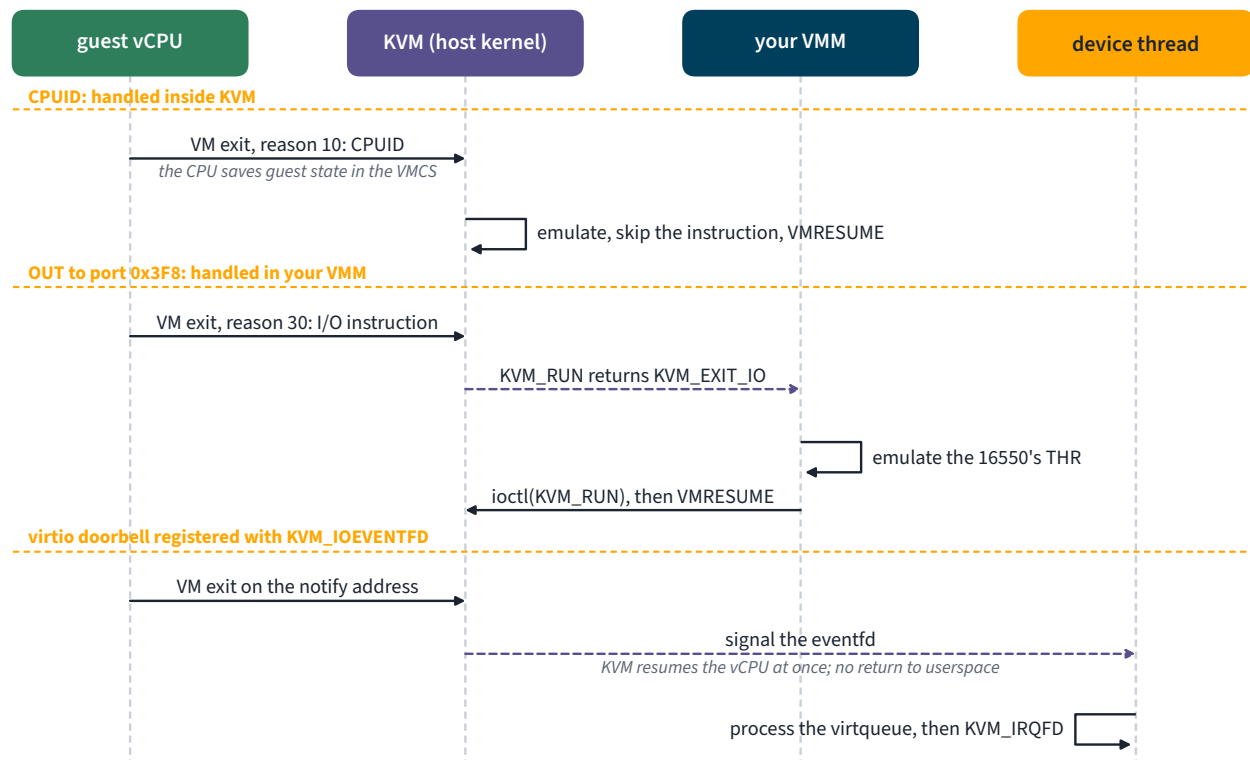
Figure 4.4.3. Where an exit is handled decides its cost: CPUID never leaves the kernel, port I/O round-trips through your VMM, and an ioeventfd doorbell wakes a device thread while the vCPU carries on.
