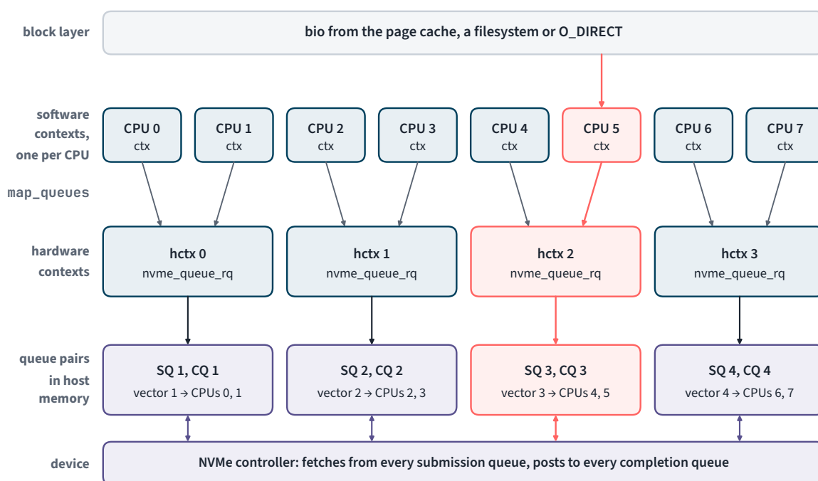
Figure 4.2.1. blk-mq with eight CPUs and four NVMe queue pairs. The highlighted request is submitted on CPU 5 and completes on CPU 4 or 5 through vector 3.
