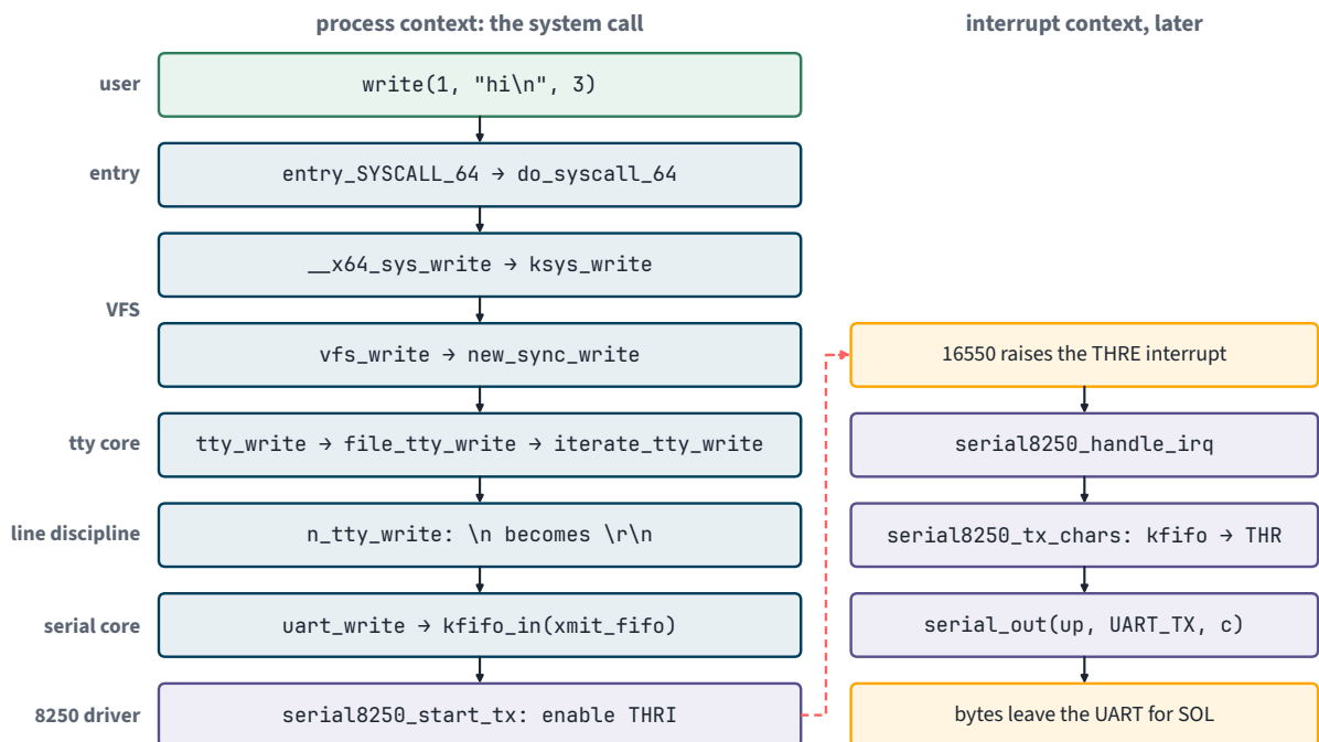
Figure 4.2.3. echo hi > /dev/ttyS1 on the server. The system call only queues bytes and enables the transmit interrupt; the 8250 interrupt handler moves them into the UART.
