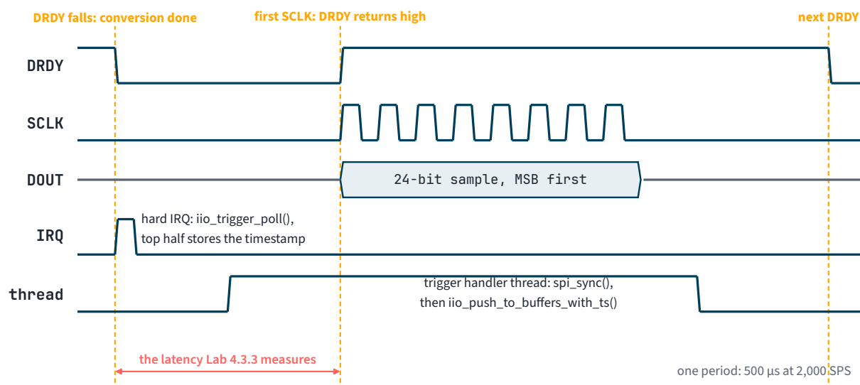
Figure 4.3.2. A data-ready trigger on the ADS1220. The hard interrupt only takes a timestamp; the delay before the first clock grows with load, and one longer than a period loses a sample.
