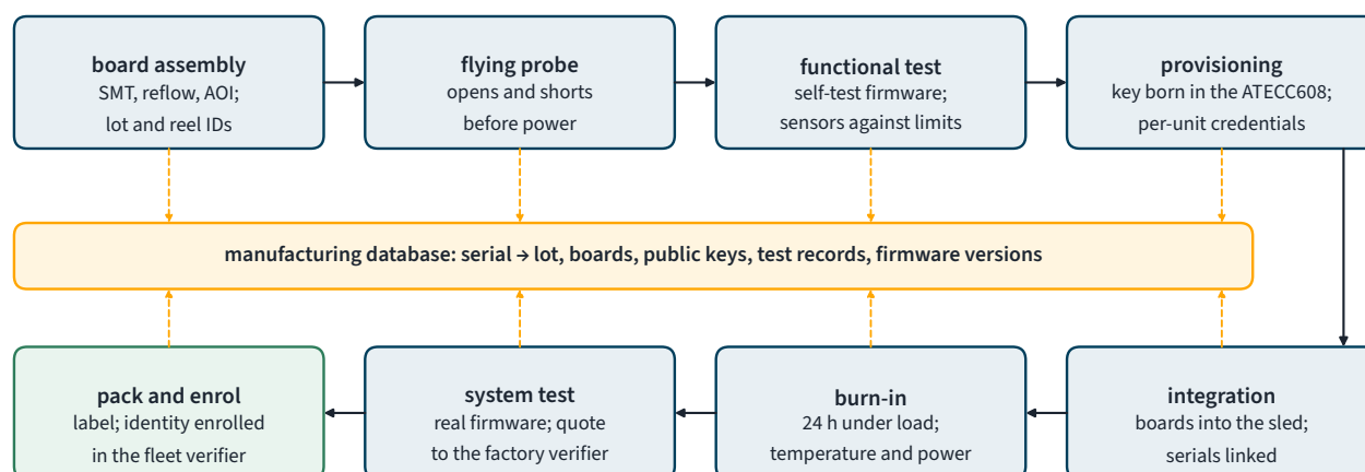
Figure 4.6.3. From bare board to enrolled module. Every station writes to the manufacturing database.
