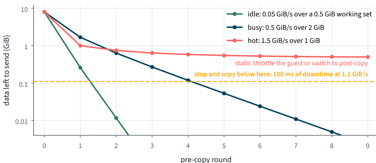
Figure 4.4.4. Pre-copy for an 8 GiB guest on a 10 Gb/s link, in a model where each round's dirty pages saturate a working set. A hot guest stalls above the downtime budget until it is throttled.
