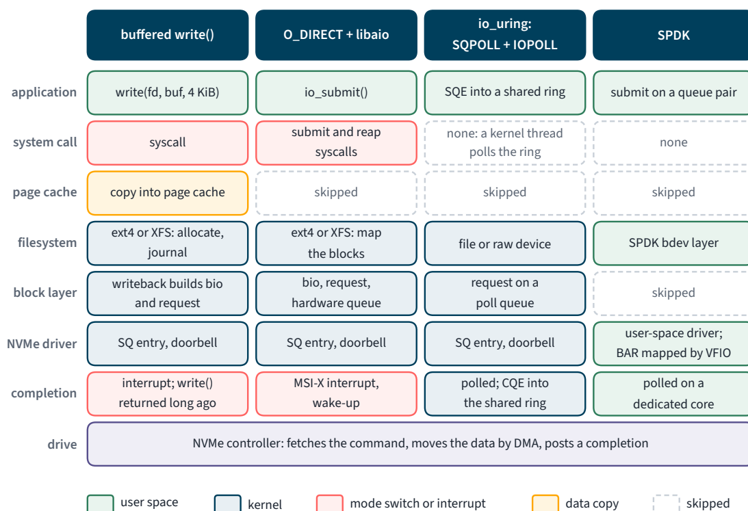
Figure 4.5.1. Four ways from a 4 KiB write to flash. Labs 4.5.1 and 4.5.2 measure what each removed layer is worth.
