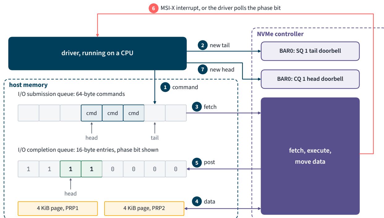
Figure 4.1.4. An NVMe read on one queue pair. The driver owns the submission queue's tail and the completion queue's head, the controller the other two; the phase bit tells the driver which completions are new on this pass.
