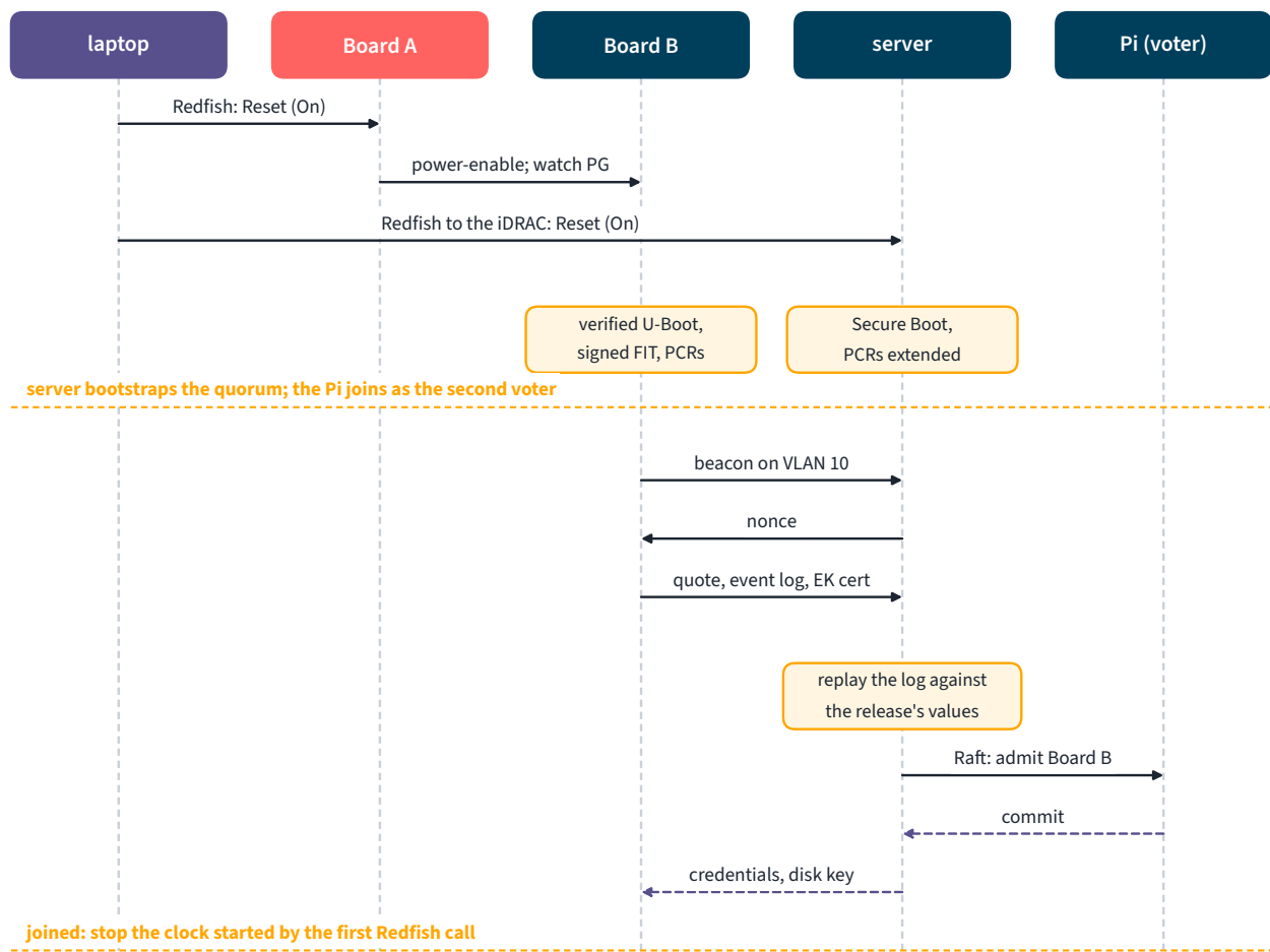
Figure 4.7.1. The cold start, from the first Redfish call to Board B's admission. The time between the first message and the last is the boot-to-joined figure your specification guessed.
