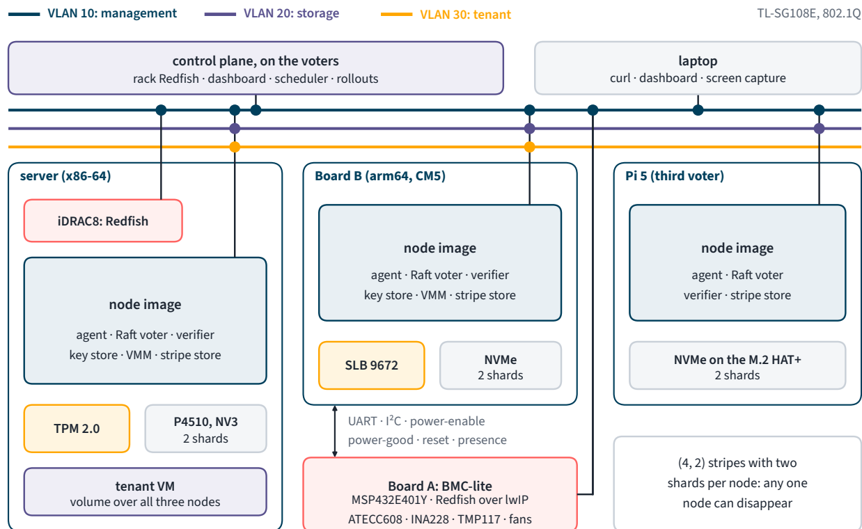
Figure 4.7.2. Module Zero on the bench: three nodes on three VLANs, with Board A on Board B's host connector and on the management VLAN through its own port. Every stripe keeps two shards on each node.
