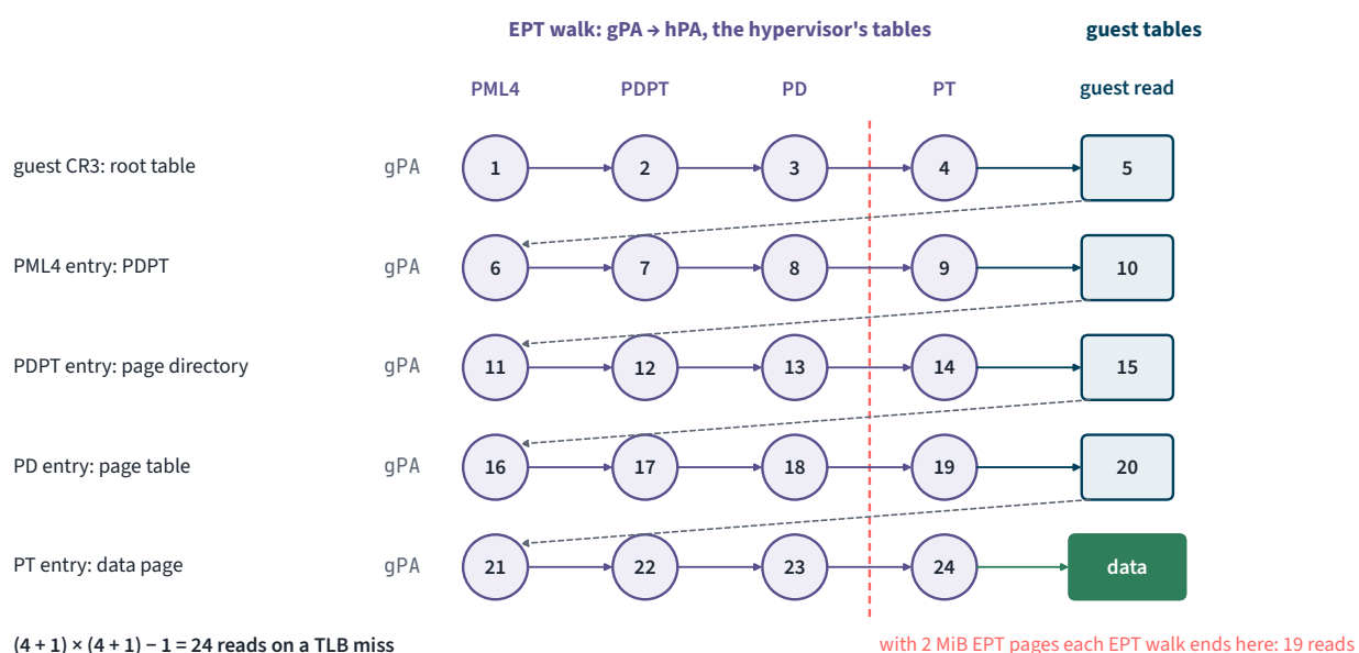
Figure 4.4.1. The two-dimensional walk. Every guest page-table pointer is a guest physical address the EPT must translate first, so four guest levels over four EPT levels cost 24 reads.
