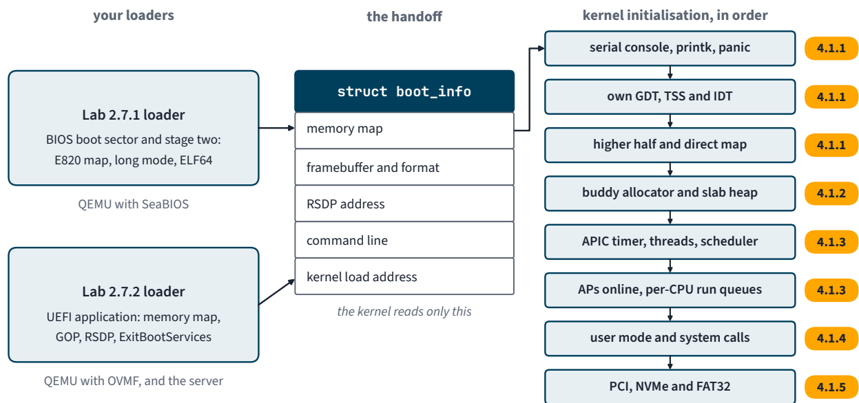
Figure 4.1.1. One kernel, two loaders. Both fill the same boot-information structure; the initialisation order on the right is the order of Labs 4.1.1 to 4.1.5.
