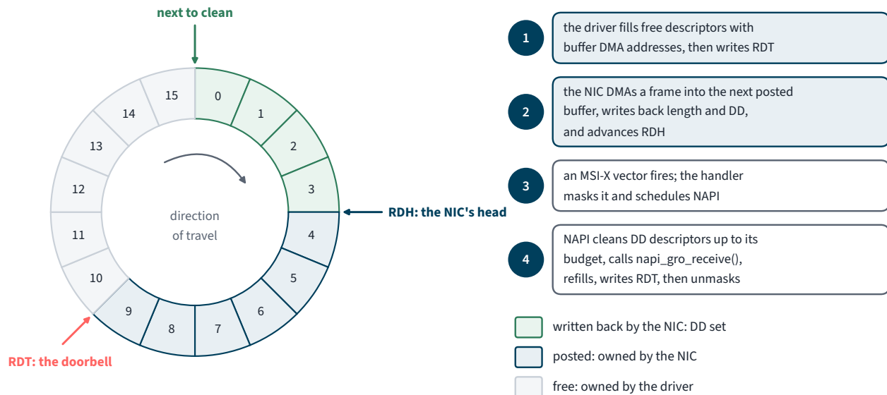
Figure 4.3.3. An RX descriptor ring in the 82599's terms: the driver posts buffers by advancing RDT, the NIC fills them and advances RDH, and NAPI cleans and refills. Lab 4.3.8 drives one.
