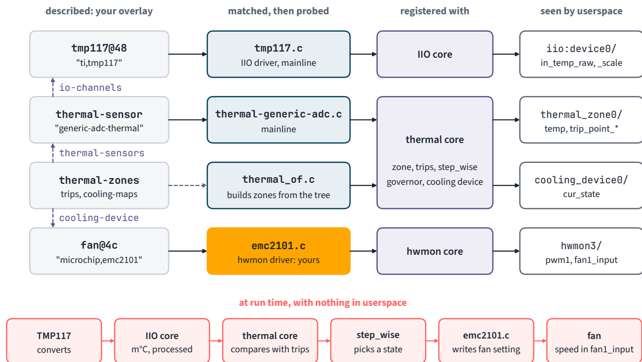
Figure 4.3.1. One overlay, three mainline drivers and yours, linked by phandles; at run time the kernel alone runs the fan curve. Lab 4.3.4 builds this.
