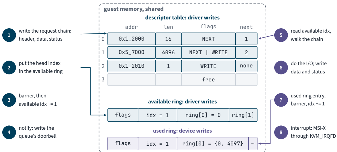
Figure 4.4.2. A virtio-blk read on a split virtqueue. The barriers stop either side seeing an index before the data it covers.
