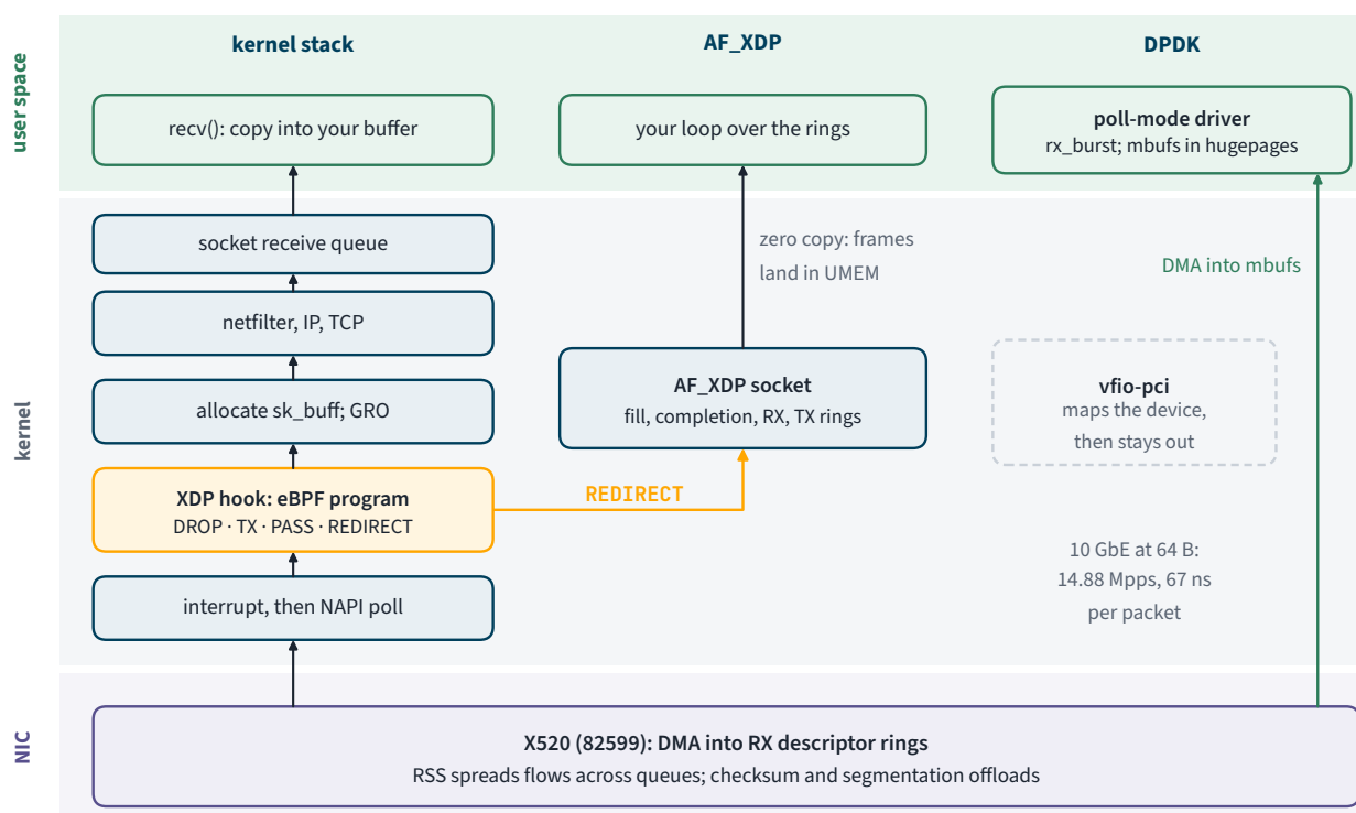
Figure 4.5.3. The receive path and its exits, each measured per core in Lab 4.5.5.
