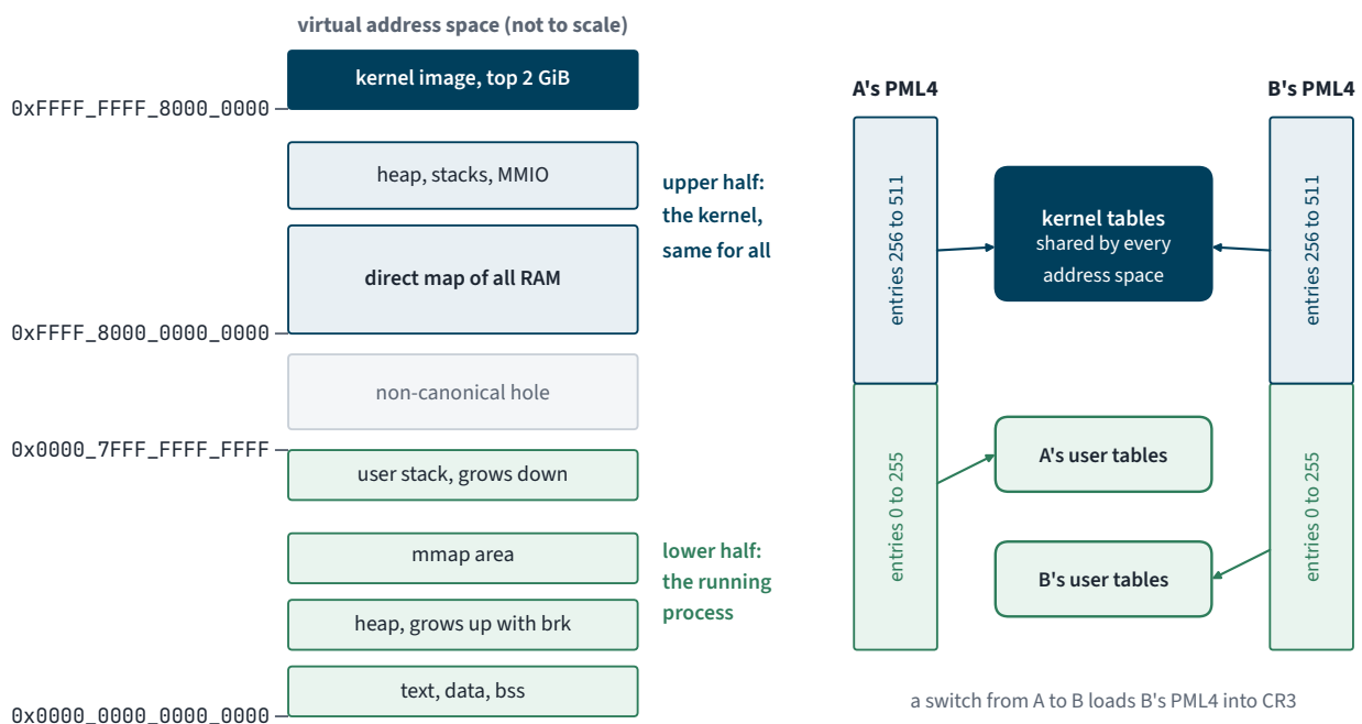
Figure 4.1.2. One possible layout for your kernel. Every PML4 points its upper 256 entries at the same kernel tables, so a context switch changes CR3 without changing the kernel's view of memory.
