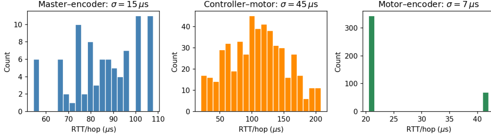
Figure 6: Per-hop RTT histograms ( x -axis in \mu\text{s} ) in a simulated airplane wing topology: one master node, three controllers, 24 motors, and 24 encoders, simulated over 30 ms. Standard deviations: master-encoder queries \sigma = 15\mu\text{s} , controller-motor loops \sigma = 45\mu\text{s} , motor-encoder loops \sigma = 7\mu\text{s} .
