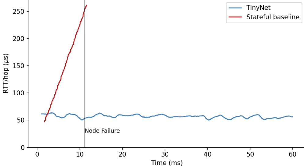
Figure 8: Per-hop RTT over time following a single node failure at t = 11 ms: TinyNet (blue) versus a stateful shortest-path baseline with a 200 ms reconvergence delay (red).
