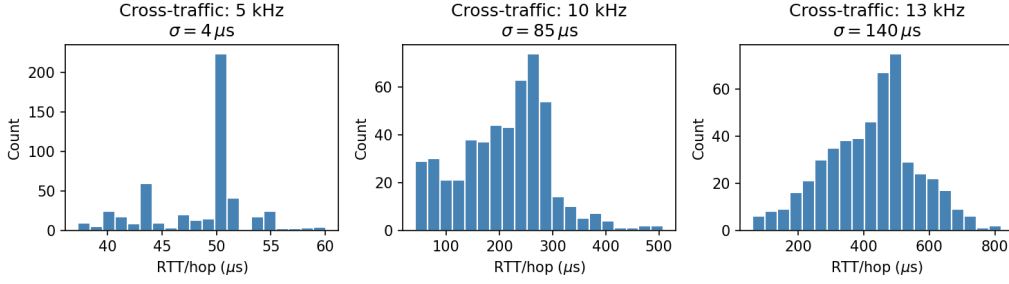
Figure 4: Histograms of Message Delay Times in a 4-by-4 Router Grid with Varying Levels of Cross-Traffic
