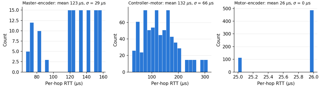
Figure 6: Per-hop RTT histograms in a simulated airplane wing topology (one master node, three controllers, eight motors, and eight encoders) in steady state ( t \geq 50\text{ ms} of a 200 ms simulation), with traffic at 20% of the nominal rates: master–encoder queries (left), controller–motor loops (center), and motor–encoder loops (right).
