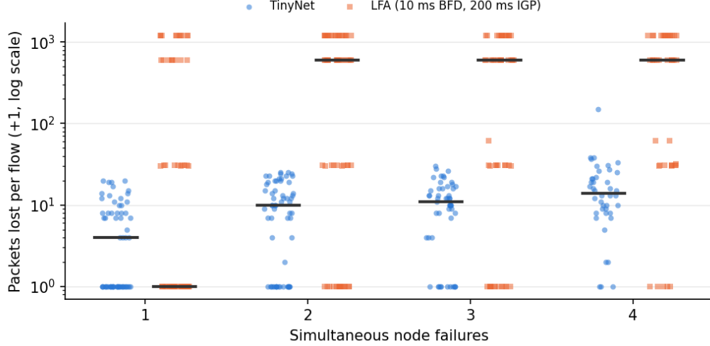
Figure 9: Packets lost per flow (plus one, log scale) after 1–4 simultaneous random node failures on the 4 \times 4 grid with a 3-kHz main flow and 6-kHz cross-traffic: TinyNet (blue circles) versus the coverage-aware LFA baseline with 10 ms BFD detection and 200 ms IGP reconvergence (orange squares). Each point is one flow in one of 30 trials per failure count; bars mark medians. Flows whose endpoints are disconnected by the failures are excluded.
