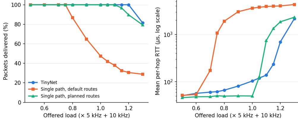
Figure 7: Delivery ratio (left) and mean per-hop RTT (right, log scale) on the 4×4 grid versus offered load, as a multiple of a 5 kHz main flow (node 0 to node 15) plus 10 kHz cross-traffic (node 3 to node 12): TinyNet (blue circles), single-path routing with the default BFS tie-break (orange squares), and single-path routing with routes planned for this traffic (aqua triangles). Each point is a 200 ms simulation; statistics use t \geq 50 ms.
