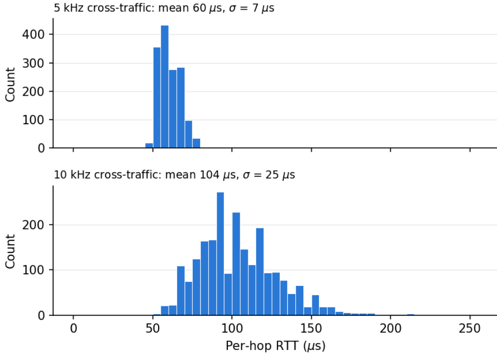
Figure 5: Per-hop RTT histograms in a 4 \times 4 grid in steady state ( t \geq 50 ms of a 200 ms simulation). Main flow: 5 kHz from node 0 to node 15. Cross-traffic on the opposite diagonal (node 3 to node 12) at 5 kHz (top) and 10 kHz (bottom).
