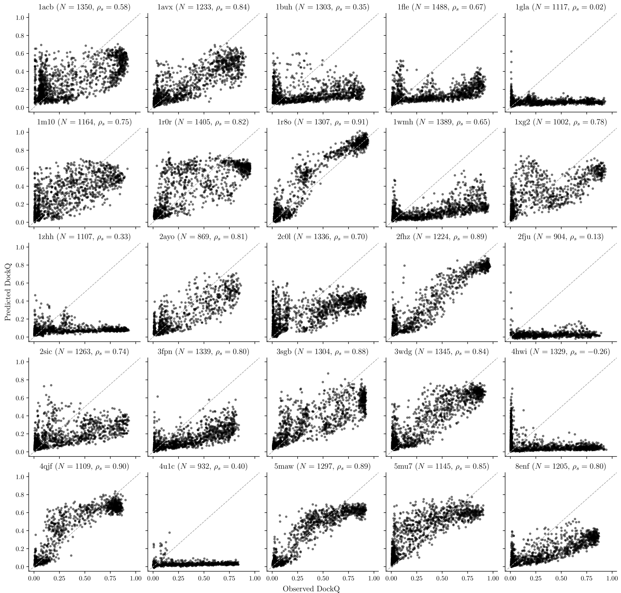
gat4_residual_02_plus_interface_node_degree
