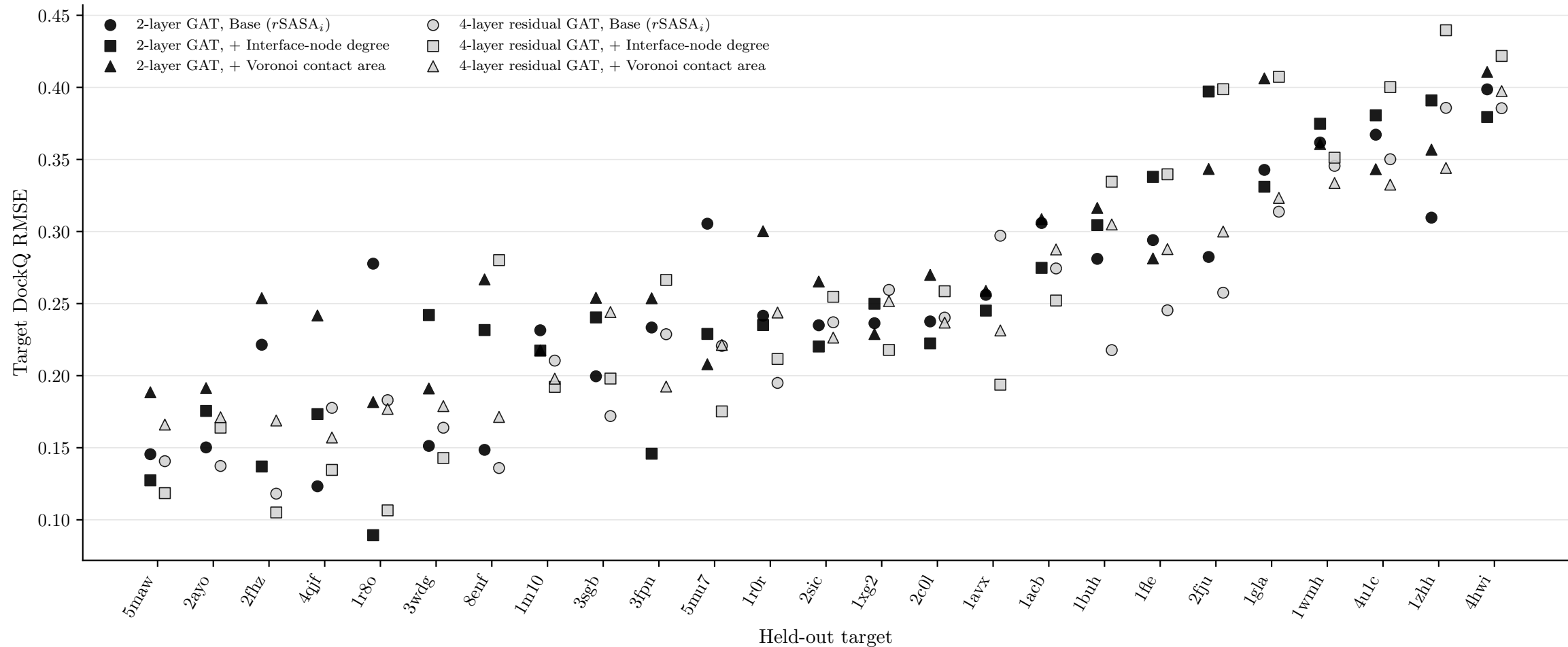
Per-target DockQ RMSE across all six runs
