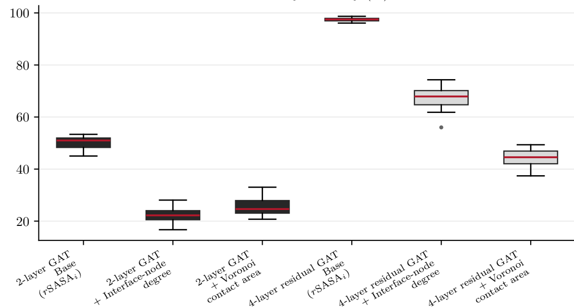
AA identity accuracy (%)
