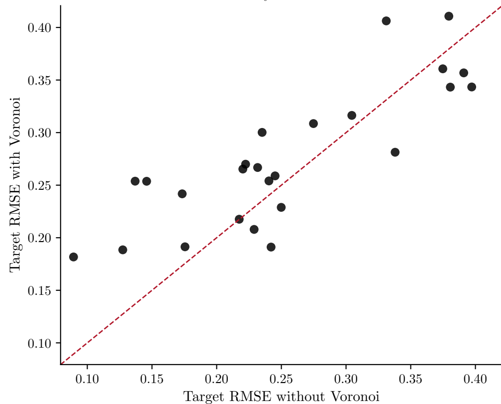
2-layer GAT
