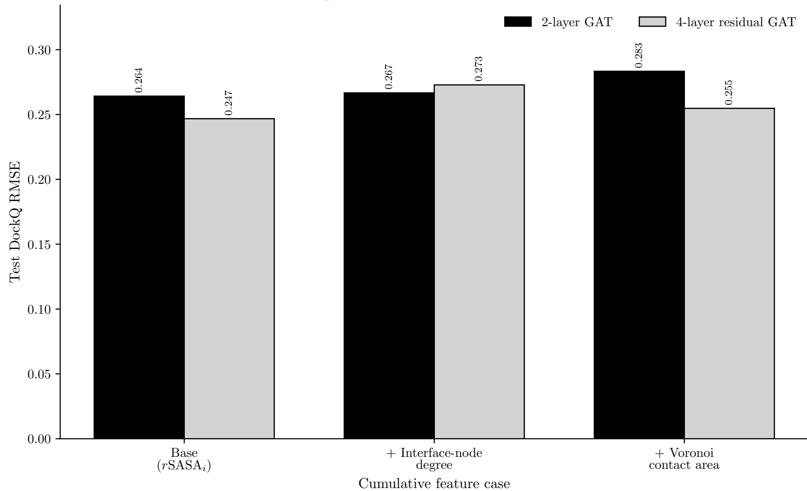
DockQ prediction error across feature additions
