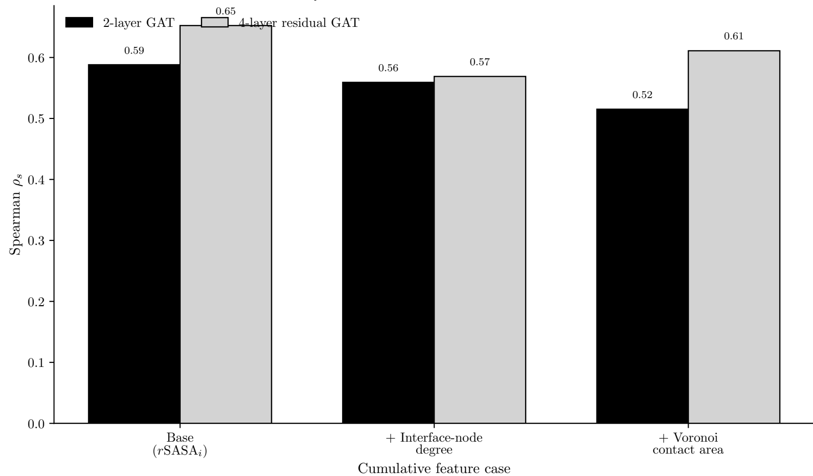
DockQ rank correlation across feature additions
