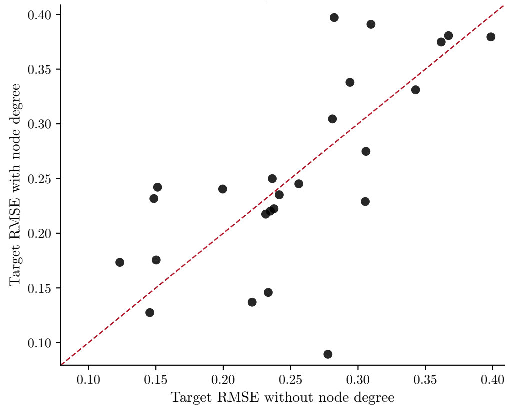
2-layer GAT
