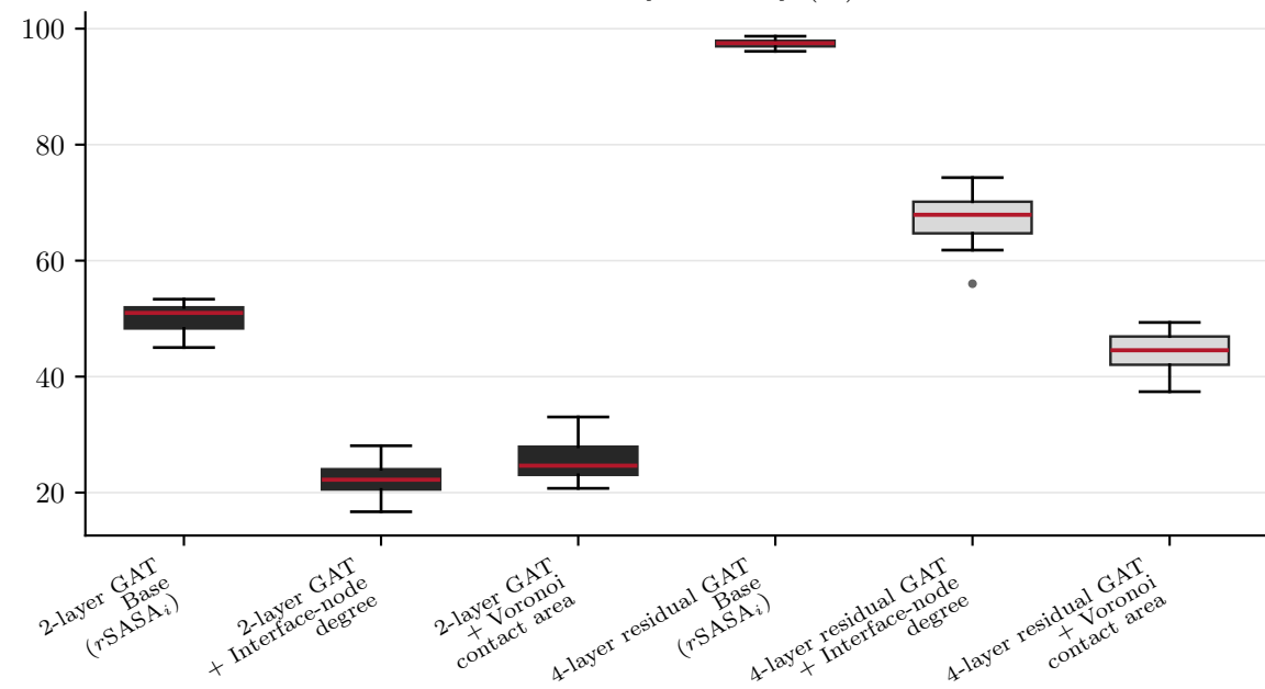
AA identity accuracy (%)
