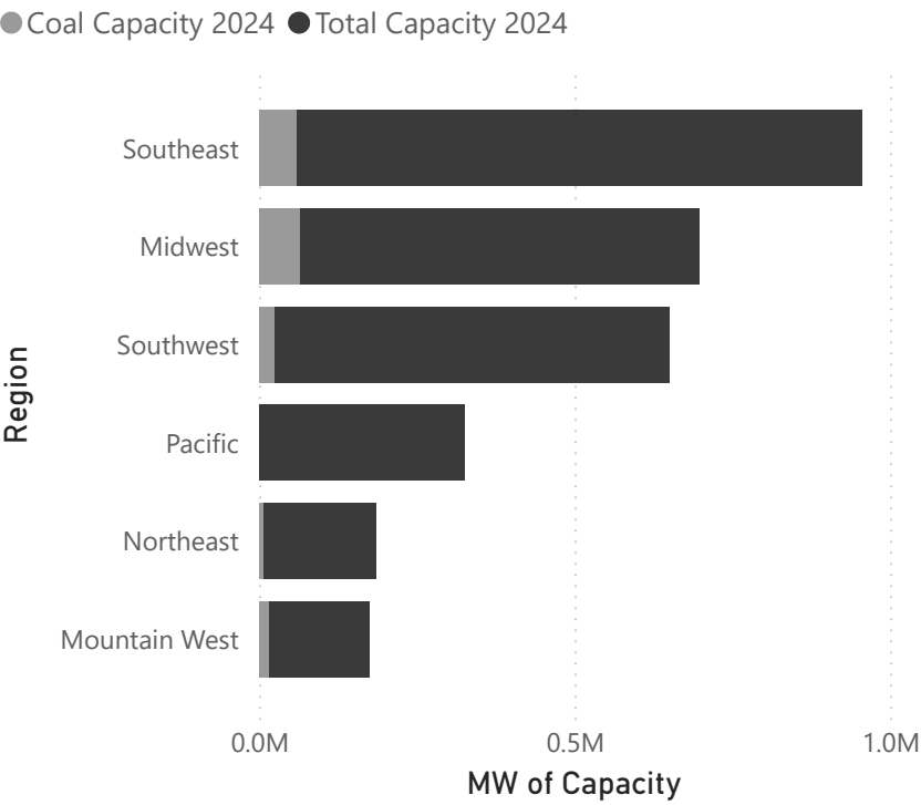
Total vs. Coal Capacity by Region (2024)
