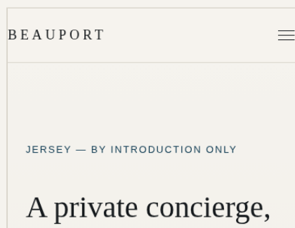
Mobile — beauport/index.html
