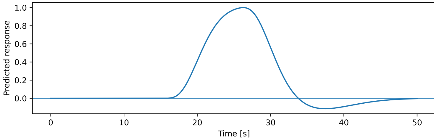
Task regressor obtained by convolution
