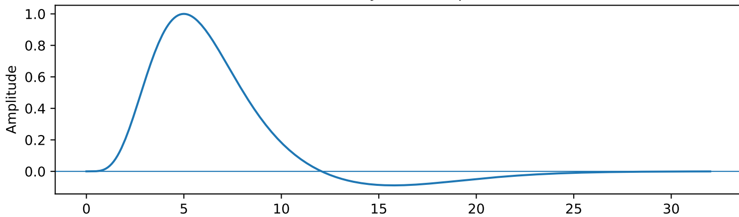
Task regressor obtained by convolution
