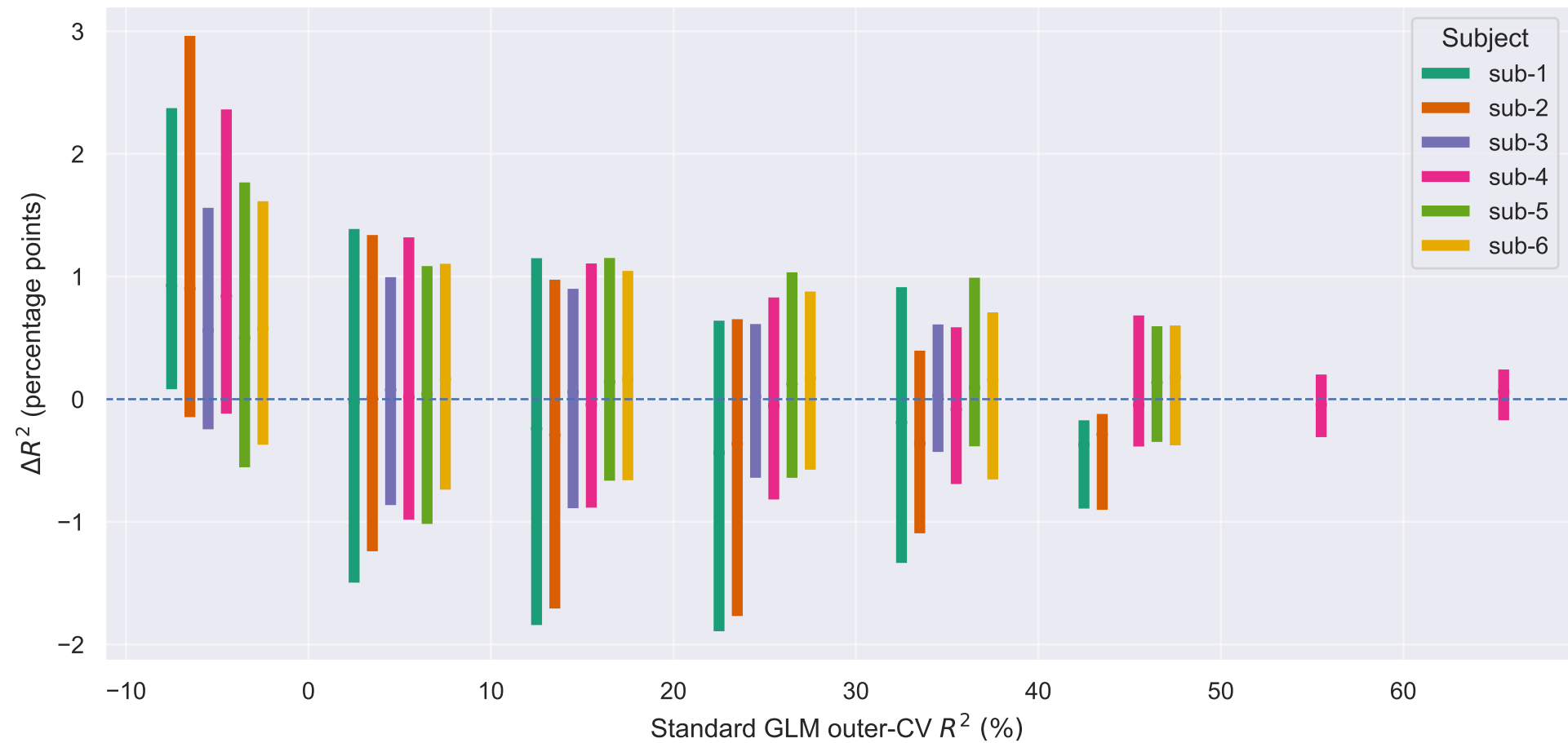
Improvement as a function of baseline accuracy: GLM + PCA
