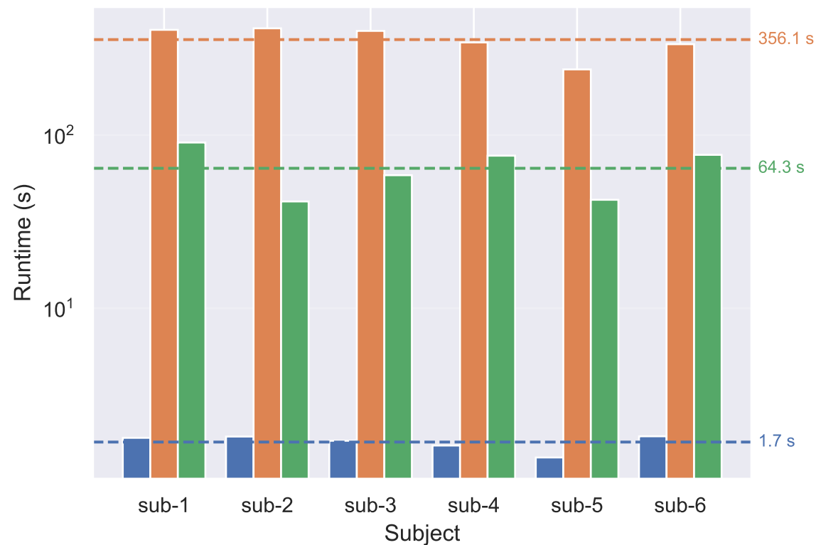
Full-data fit
