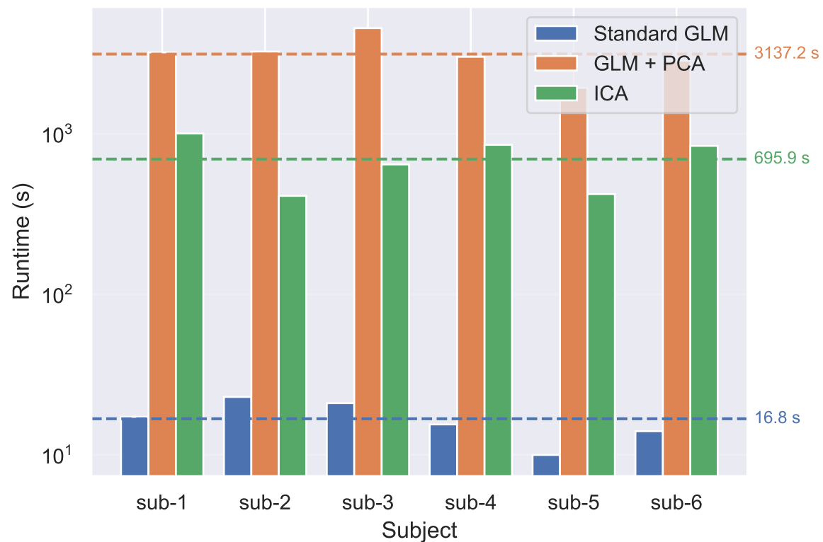
Outer-CV benchmark
