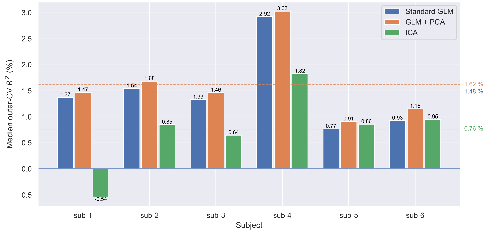
Median prediction accuracy across subjects
