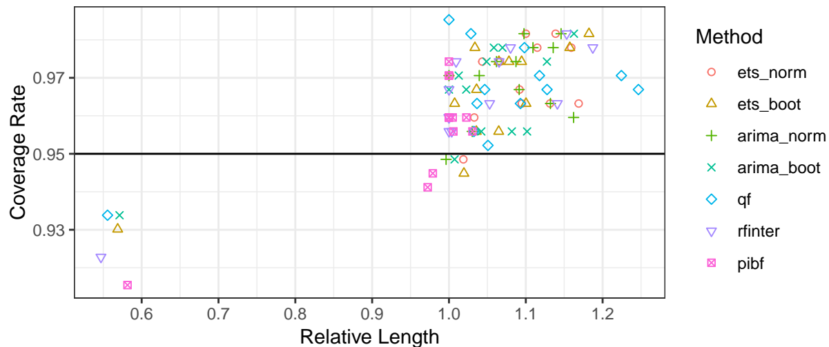
95% prediction intervals
