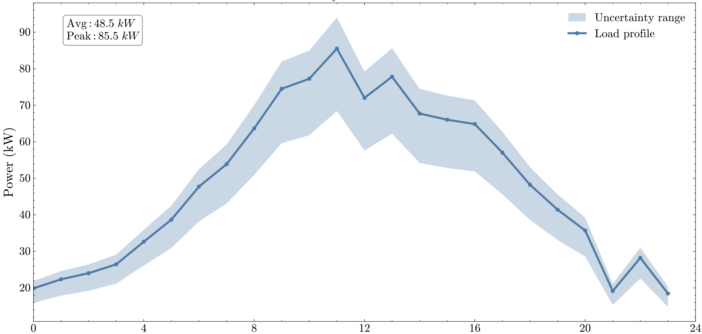
Daily Load Profile
