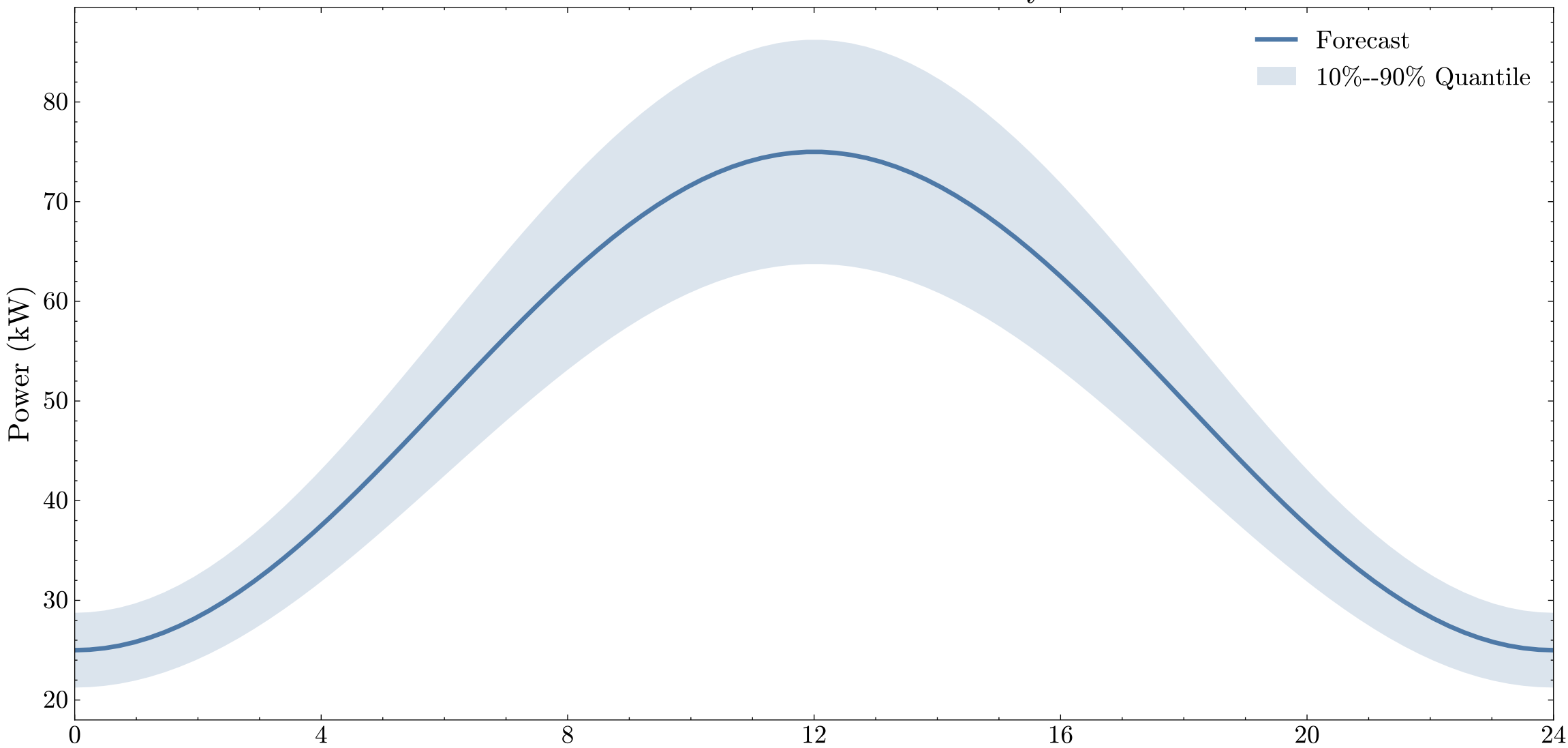
Load Forecast with Uncertainty
