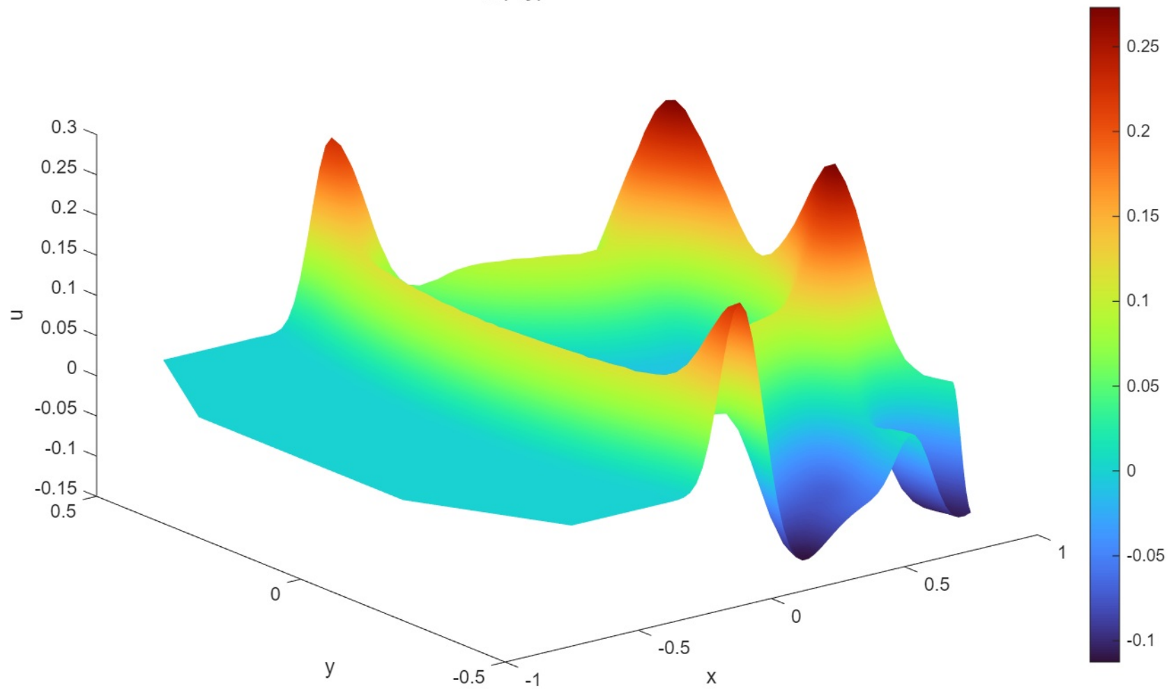
u_{2.5}(x,y) - Neumann
