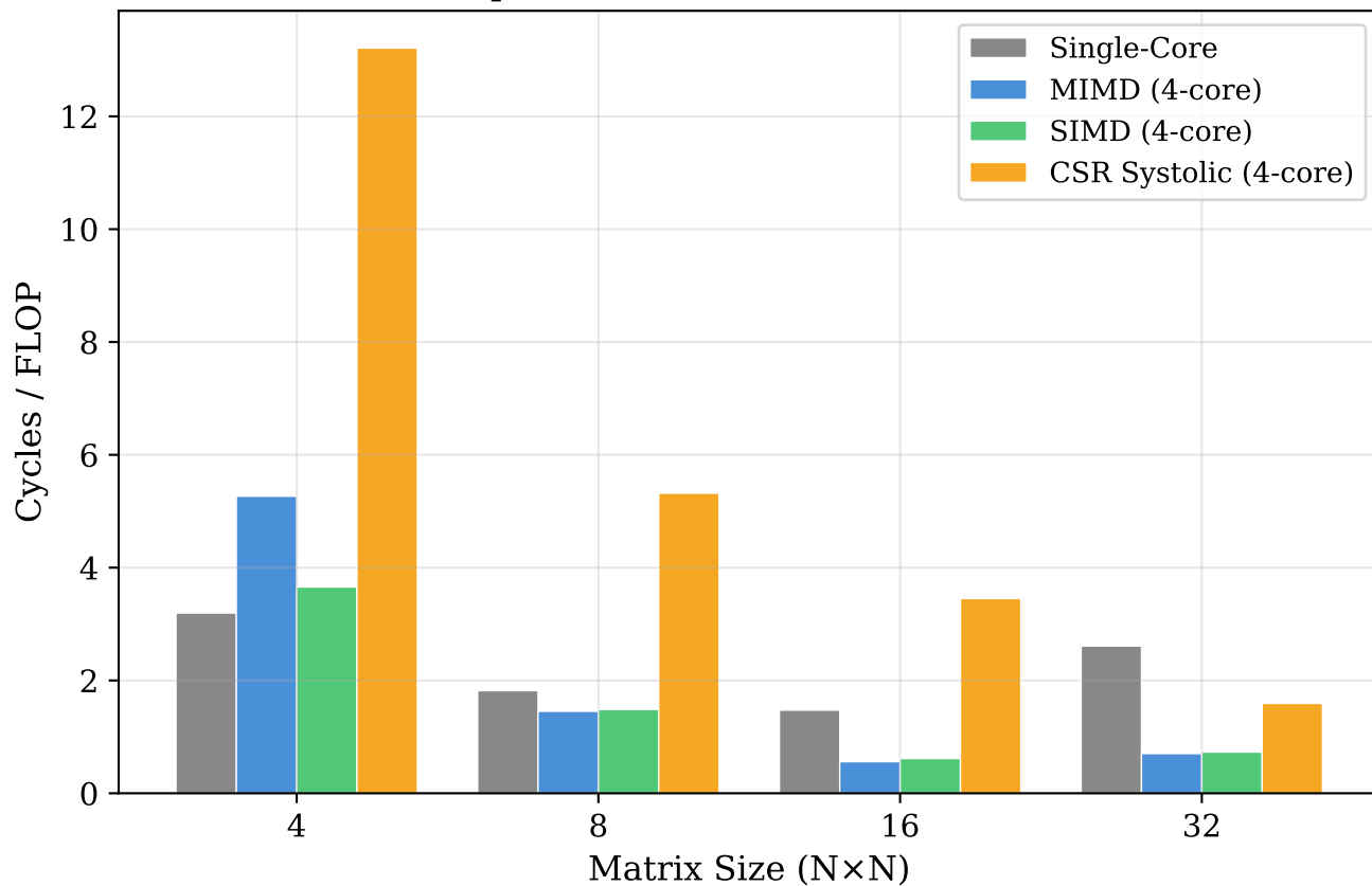
Compute Utilization (lower = better)
