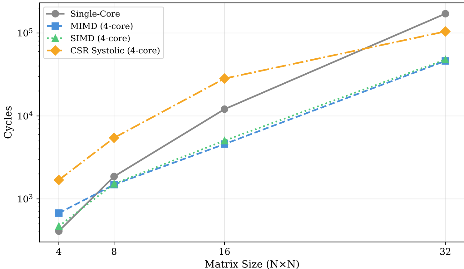
GEMM Execution Cycles by Mode (lower is better)
