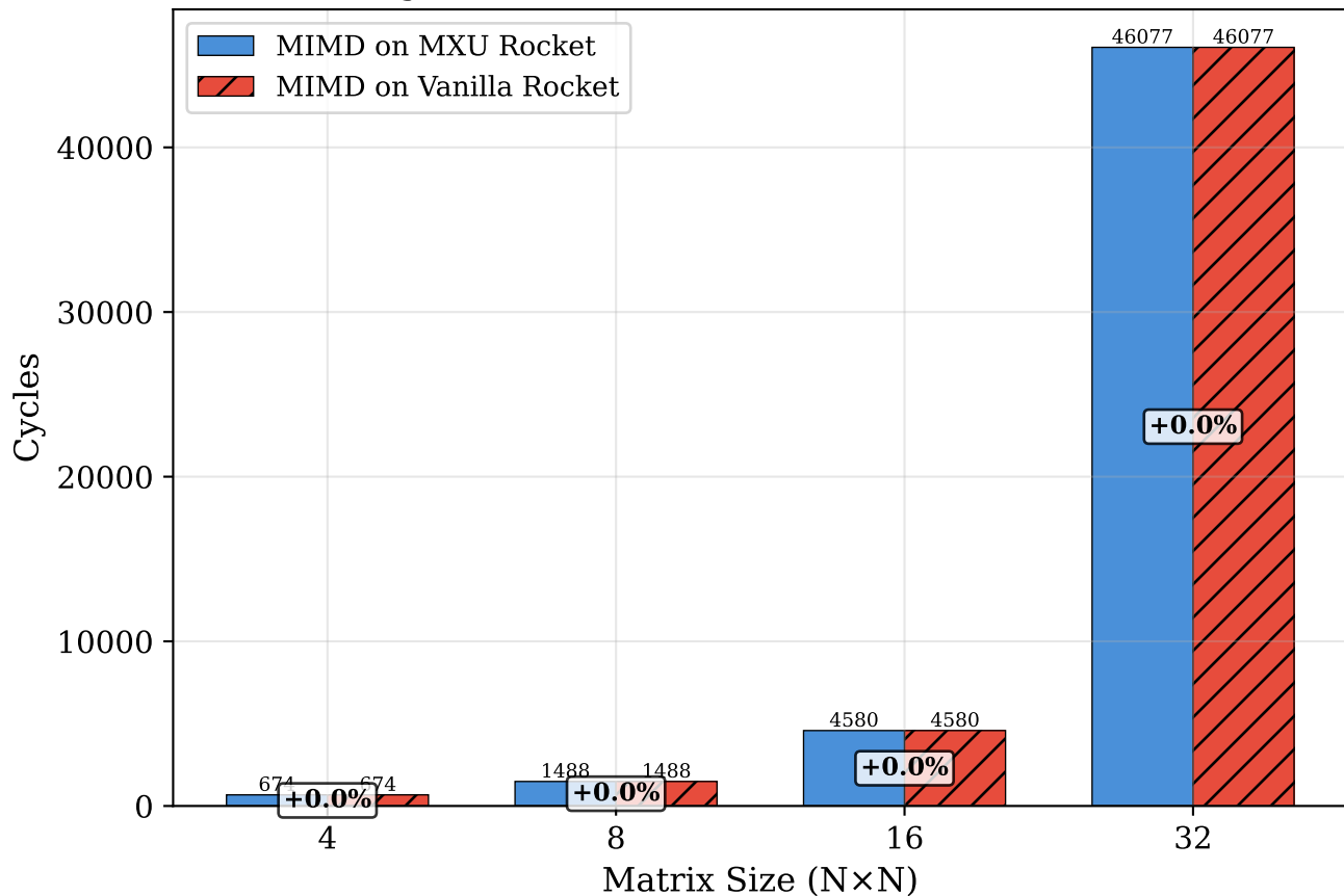
MIMD Regression: MXU vs Vanilla Rocket (lower is better)
