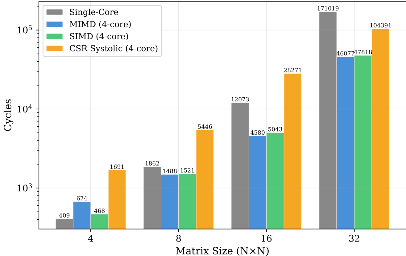
GEMM Execution Cycles by Mode
