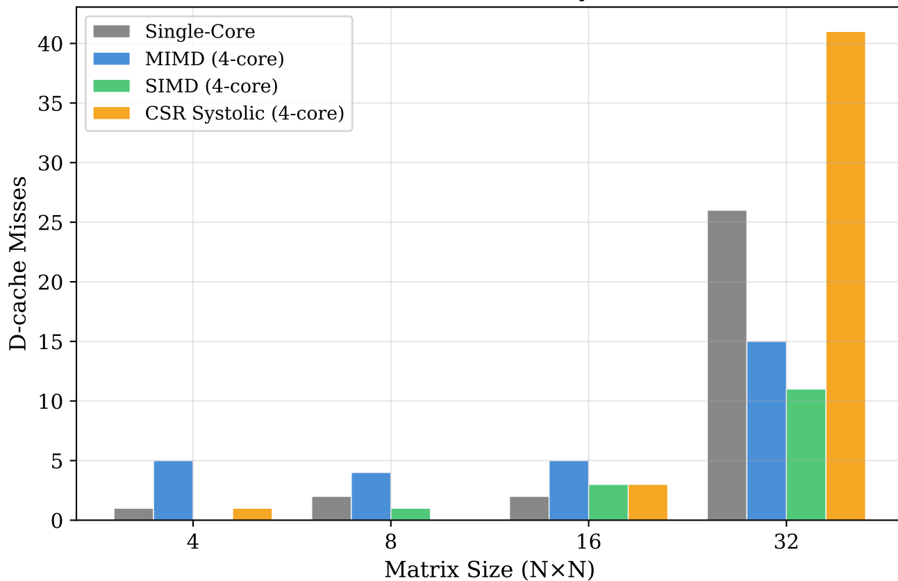
D-cache Miss Count by Mode
