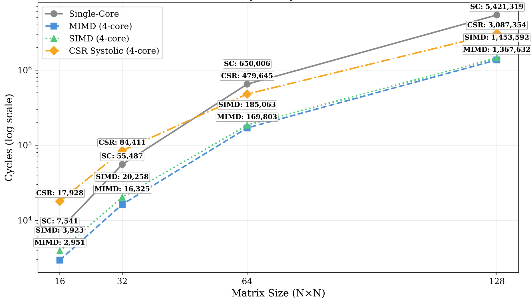
SGEMM Execution Cycles by Mode (lower is better)
