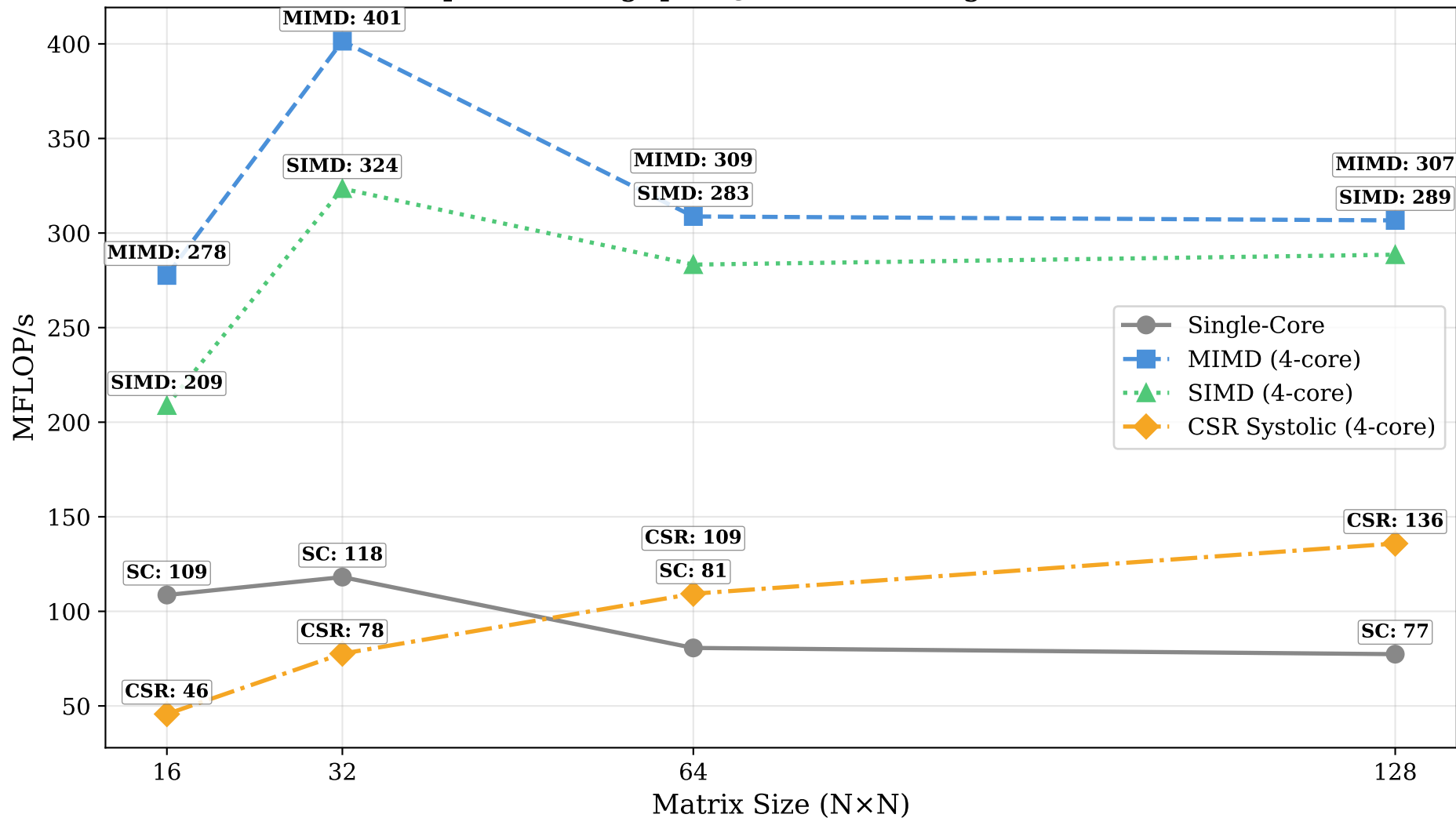
Compute Throughput @ 100 MHz (higher is better)
