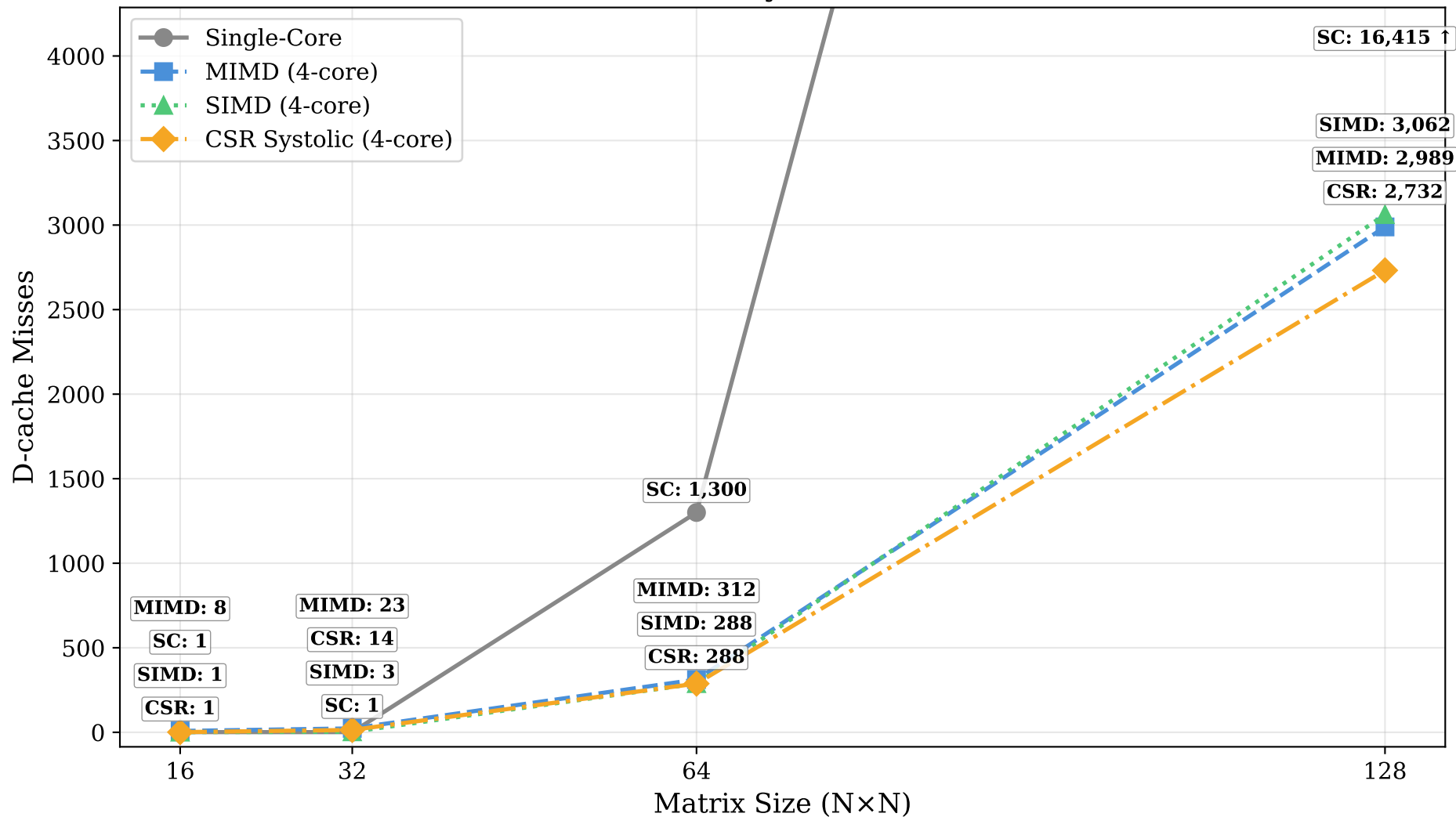
D-cache Miss Count by Mode (lower is better)
