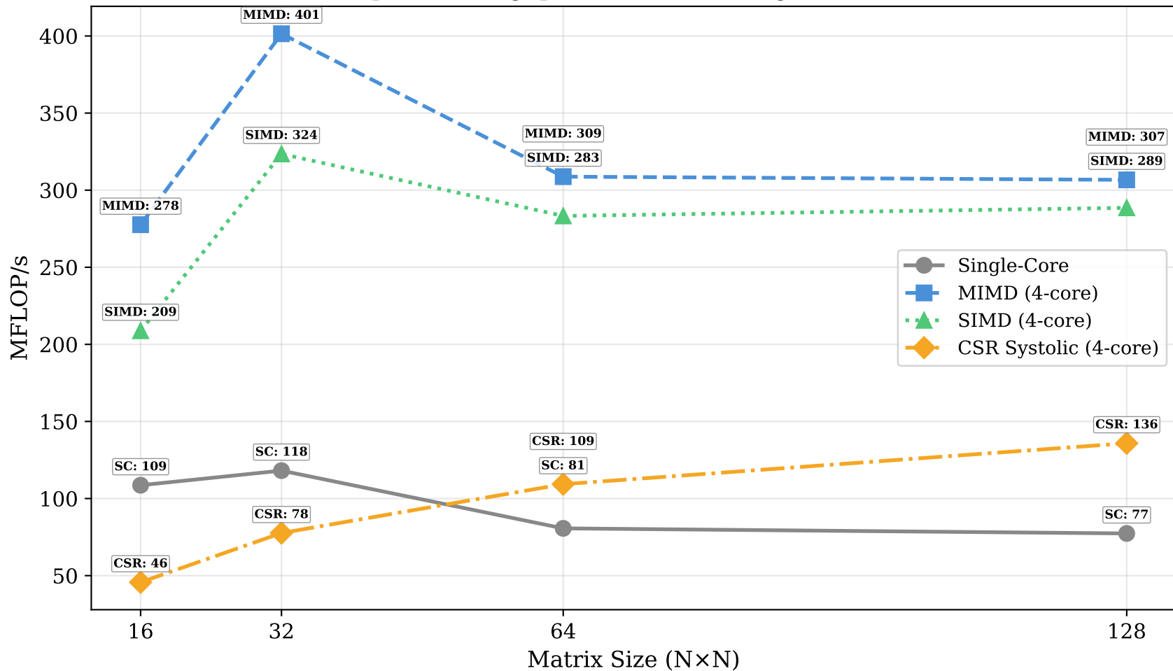
Compute Throughput @ 100 MHz (higher is better)
