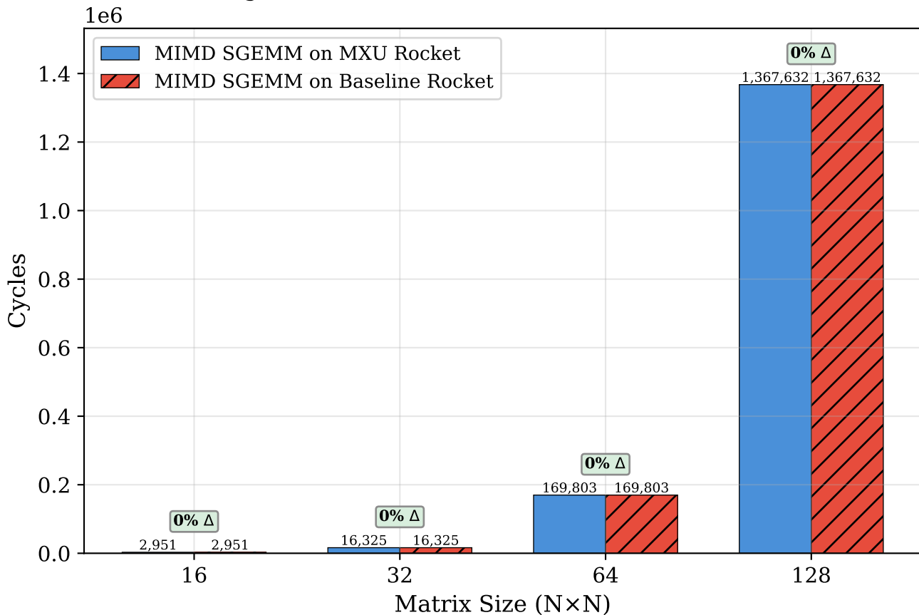
MIMD Regression: MXU vs Baseline Rocket (lower is better)
