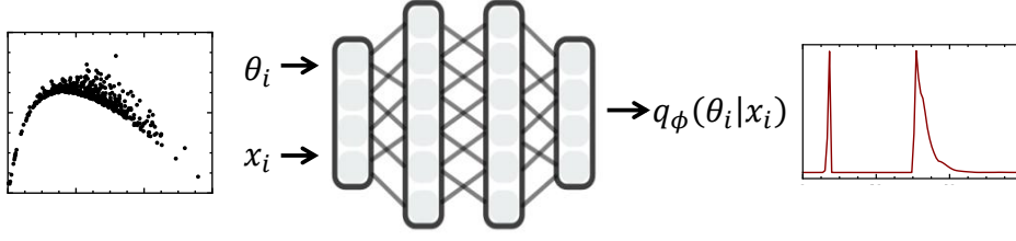
Figure 3: Training of the neural network in SBI from the example of an angled throw. The network learns to map the tuples (\theta_i, x_i) to the estimated posterior density q_\phi(\theta_i | x_i) . Parts of the figure are adapted from Deistler et al. (2025) .
