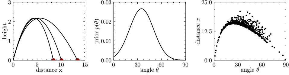
Figure 2: Simulations in SBI from the example of an angled throw. Left: simulation of throw trajectories, Center: prior distribution of parameters \theta_i , Right: simulated dataset (\theta_i, x_i) . The example is adapted from Deistler et al. (2025) .
