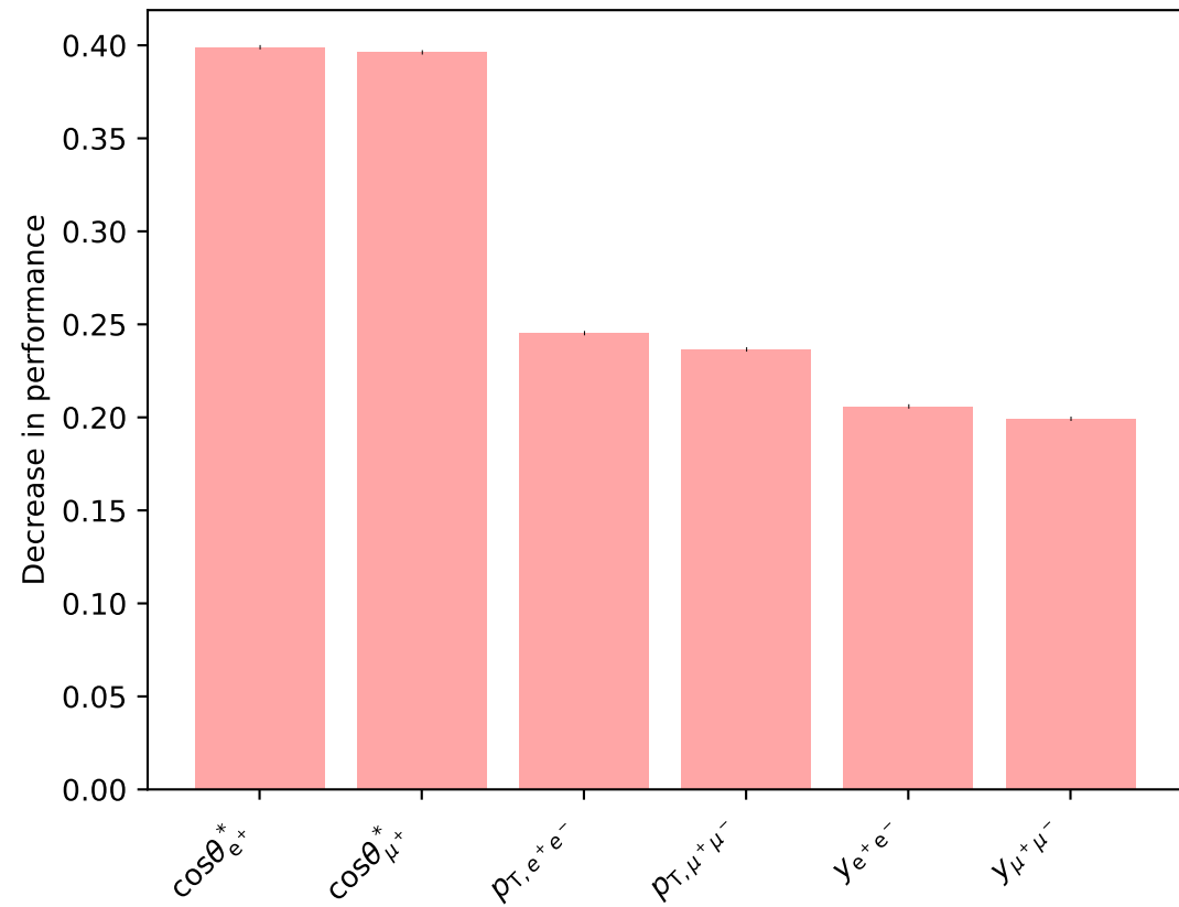
Permutation importance for RFR ct (NLO QCD, LHE, fiducial)
