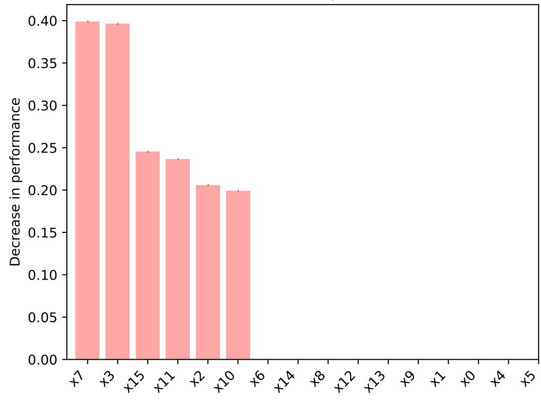
Permutation importance for RFR ep (NLO QCD, LHE, fiducial)
