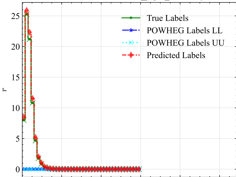
Predicted vs. True Labels - FFNN_paper_4extraLayers
