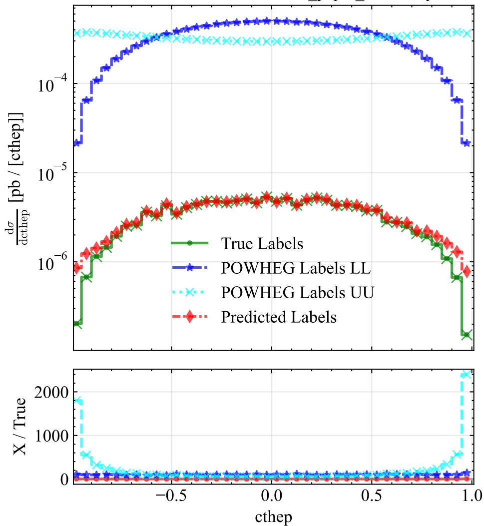
Predicted vs. True Labels - FFNN_paper_4extraLayers
