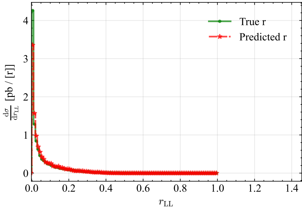
16 Predicted vs. True Labels - FFNN_paper_4extraLayers
