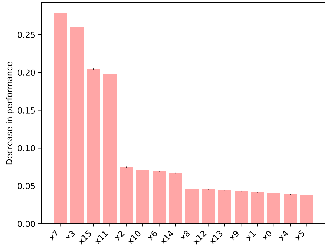
Permutation importance (NLO QCD, LHE, fiducial)
