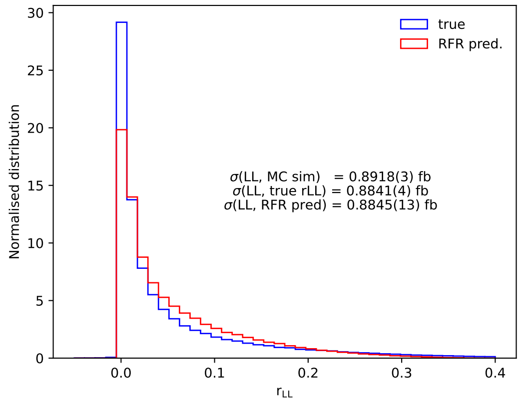
r_{LL} label (NLO QCD, LHE, fiducial)
