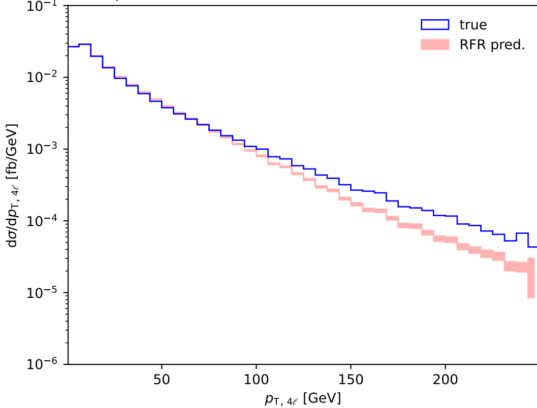
Four-lepton transverse momentum (NLO QCD, LHE, fiducial)
