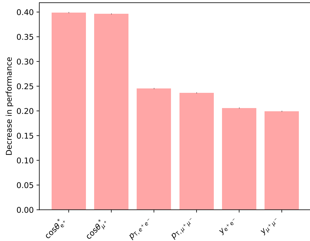
Permutation importance (NLO QCD, LHE, fiducial)
