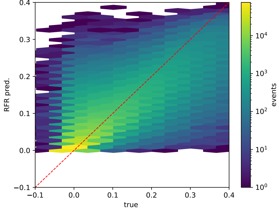
True vs pred. r_{LL} labels (NLO QCD, LHE, fiducial)
