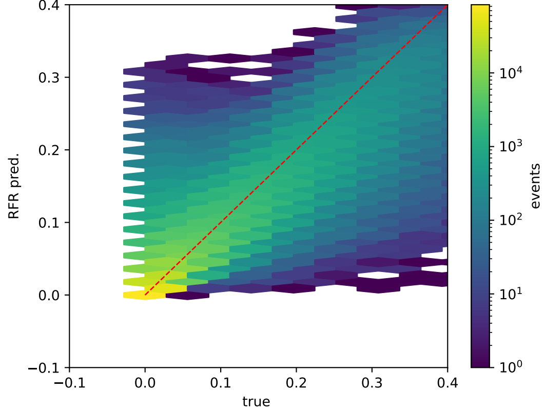
True vs pred. r_{LL} labels (LO, fiducial)
