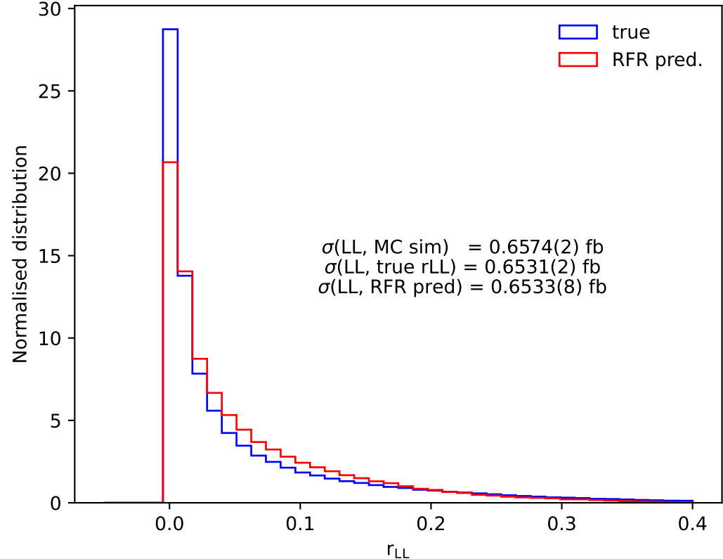
r_{LL} label (LO, fiducial)
