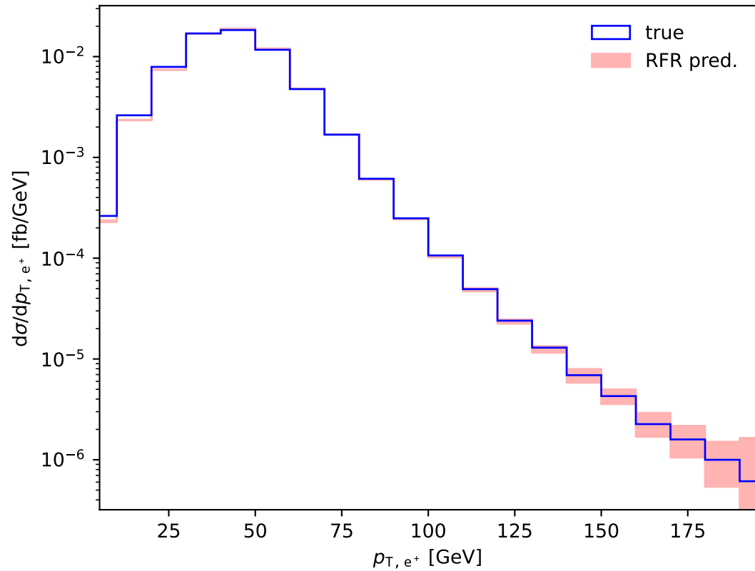
Positron transverse momentum (LO, fiducial)
