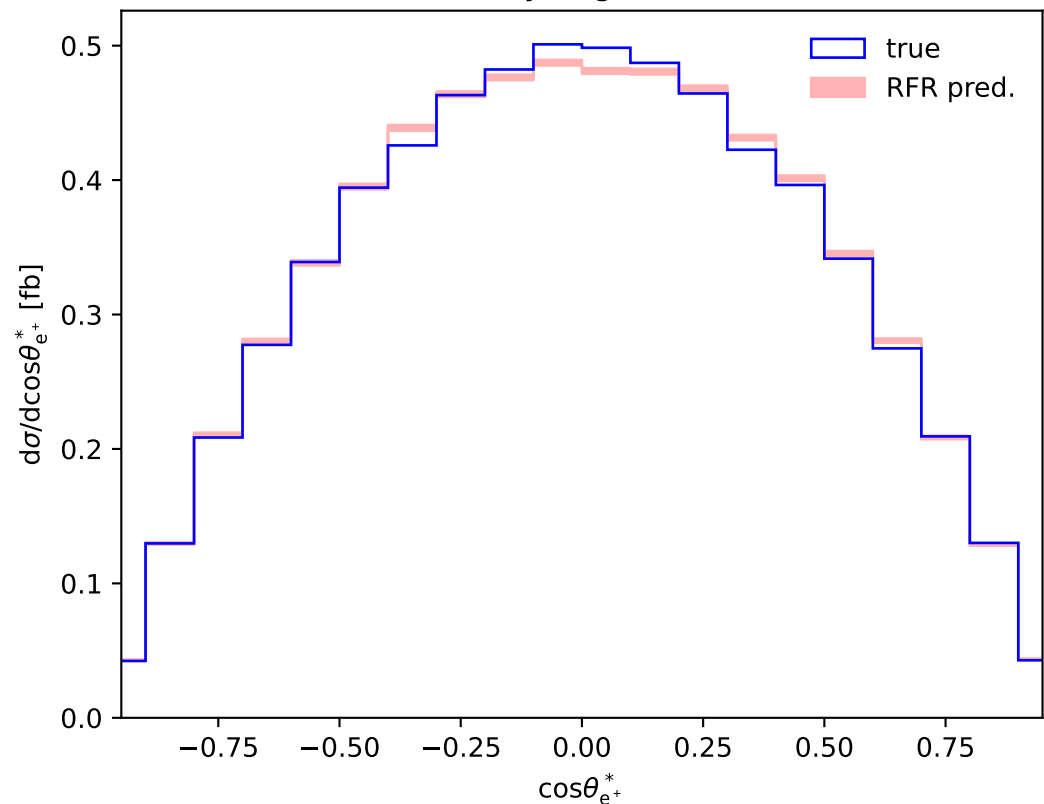
Positron decay angle (LO, fiducial)
