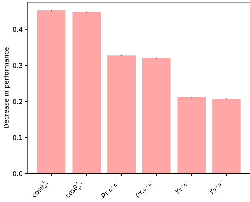
Permutation importance (LO, fiducial)
