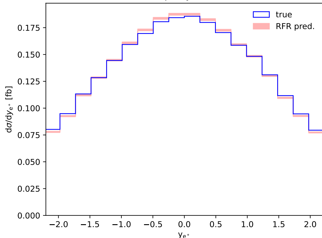
Positron rapidity (LO, fiducial)
