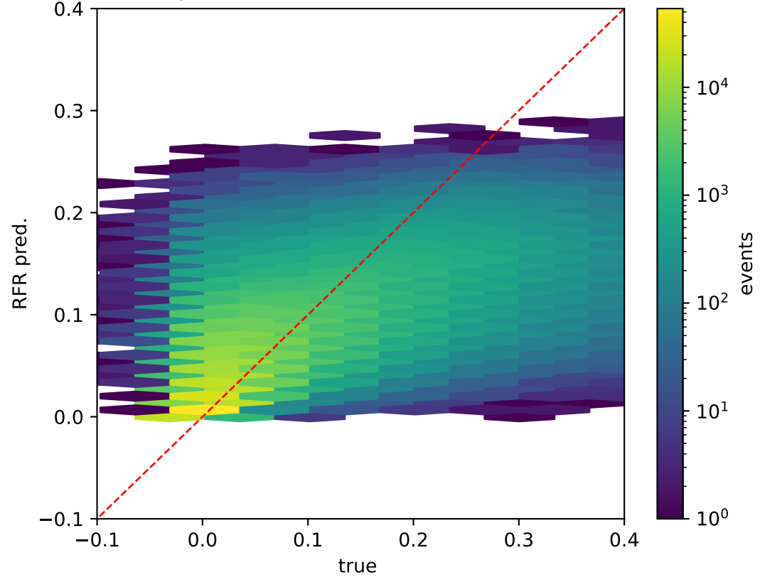
True vs pred. r_{LL} labels (NLO QCD, LHE, fiducial)
